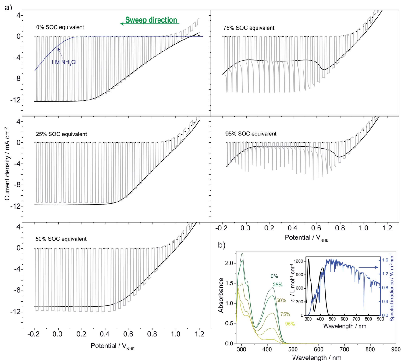
Fig. 5 (a) LSVs recorded on \text{pn}^+\text{Si}/\text{TiO}_2 in 0.4 M ferro/ferricyanide solutions in ratios matching that expected for different SOCs in the solar flow battery (SOC equivalents) and of the pure supporting electrolyte (1 M \text{NH}_4\text{Cl} displayed with the 0% SOC equivalent, blue line) relative to a reference electrode. Recorded in constant light (1 sun, full black line), chopped (full grey line) and dark (dotted black line behind chopped). (b) The measured absorbance of the SOC equivalent solutions (diluted 300 times) and the inset shows the calculated associated extinction coefficient (black) overlaid on the AM1.5G spectrum (blue) (see S7 † ). 27
