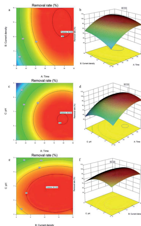
Fig. 5 Contour and surface plots showing the relationship between the removal of fluoride (%) and independent parameters: (a and b) time–current density, (c and d) time–initial pH, and (e and f) initial pH–current density.
