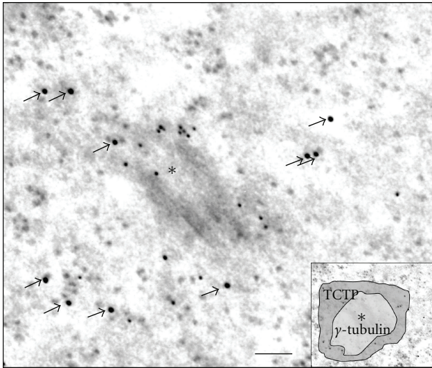
FIGURE 6: Double labeling of \gamma -tubulin and TCTP in the centrosome of Xenopus laevis oogonium. Centriole labeled with black asterisk; 18 nm gold particles (black arrows) correspond to the presence of TCTP, small, and 10 nm gold particles around the centriole mark the presence of \gamma -tubulin. Inset in the bottom right corner shows the central area around the centriole where \gamma -tubulin is present (clear central area), and the TCTP-containing external area of the centrosome (dark grey). Bar is equal to 100 nm.
