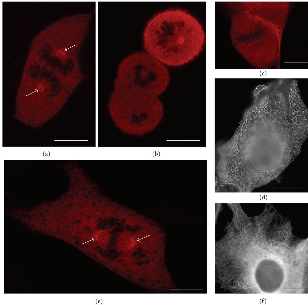
FIGURE 2: Expression of Myc-XITCTP in Xenopus laevis XL2 cells. (a) Confocal section of XL2 cell in anaphase with high concentration of XITCTP at the spindle poles (white arrows). (b) Confocal section of two dividing XL2 cells with high concentration of XITCTP at the spindle poles. (c) Control mitotic XL2 cells expressing Myc tag only. (d) Interphase XL2 cell expressing Myc-XITCTP. XITCTP is localized in distinct fibers in the cytoplasm. (e) Mitotic murine NIH3T3 cell expressing Myc-XITCTP. High concentration of XITCTP is present at the spindle poles (white arrows). (f) Interphase murine NIH3T3 cells expressing Myc-XITCTP. Note that XITCTP forms MT-like fibers in the cytoplasm. Bar is equal to 20 \mu\text{m} .
