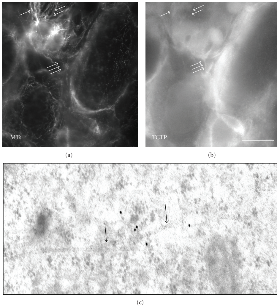
FIGURE 4: MTs and TCTP in Xenopus laevis tadpole ovary. Interphase cells. Upper panel, left: \beta -tubulin, right: TCTP localization. Anti-XITCTP was used for this localization. Single white arrow points to cellular structures positive both for \beta -tubulin and TCTP. Double arrows point to \beta -tubulin-positive and TCTP-negative fibers. Triple arrows point to TCTP-positive and \beta -tubulin-negative fibers. Bar is equal to 20 \mu\text{m} ; Bottom panel: electron microscopy gold immunolabeling of TCTP (black particles in the center) in the vicinity of MTs (black arrows). Bar is equal to 100 nm.
