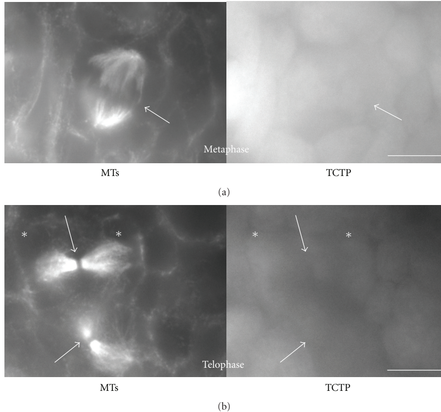
FIGURE 5: MTs and TCTP in mitotic Xenopus laevis oogonia. Left: \beta -tubulin, right: TCTP localization in tadpole oogonia. Anti-XITCTP was used for this localization. Upper panel: metaphase cell. Left: mitotic spindle visualized by \beta -tubulin staining (white arrow). Right: The whole of the spindle is positive for TCTP (white arrow). Bottom panel: two telophase oogonia. Left: prominent midbodies are visualized by anti- \beta -tubulin immunofluorescence (white arrows). White asterisks show the position of two daughter cells. Note the absence of TCTP in the midbodies. Bar is equal to 20 \mu m.
