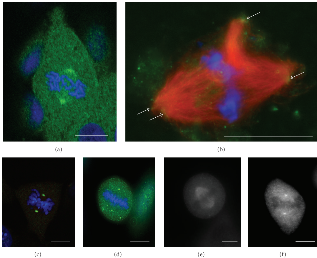
FIGURE 1: Immunofluorescence localization of TCTP in Xenopus laevis mitotic spindles using XITCTP antibody. (a) Confocal section of an XL2 cell showing the presence of TCTP in the spindle with higher density at the spindle poles. (b) Isolated spindle formed by sperm-head addition to the CSF extract. Red MTs stained with rhodamine- \beta -tubulin added to the extract, green TCTP detected by immunofluorescence with XITCTP antibody. White arrows point to spindle poles with TCTP staining. Blue DNA stained with DAPI. Note the presence of yellow staining of TCTP at the spindle poles and the absence of TCTP in the remaining parts of the spindle. (c) Confocal section of murine metaphase NIH3T3 cell stained with XITCTP antibody (green) and with DAPI for DNA. Note that XITCTP stains exclusively two distinct spots corresponding to the centrosomes, at the spindle poles corresponding. (d) Confocal section of human HeLa metaphase cell. Green TCTP detected with XITCTP antibody, blue DNA. XITCTP stains two spindle poles; the granular background staining is also visible in the cytoplasm. (e) Human HeLa metaphase cell. Green TCTP detected with homologous HsTCTP antibody, blue DNA. HsTCTP stains the whole spindle. (f) Monkey Cos7 metaphase cell incubated with anti-rat TCTP antibody showing a very distinct staining of spindle poles. Bar is equal to 20 \mu\text{m} .
