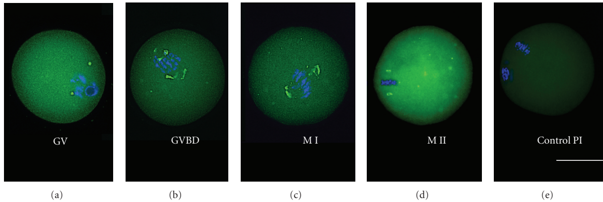
FIGURE 3: Immunofluorescence localization of TCTP with anti-XITCTP antibody in mouse maturing oocytes. GV: prophase I-arrested oocyte, GVBD: the beginning of maturation, MI and MII: oocytes in MI and MII phase of meiosis, respectively, control PI: control MII oocyte stained with the preimmune serum. XITCTP antibody stains PCM in all stages of maturing mouse oocytes. DNA (blue) stained with DAPI. Bar is equal to 40 \mu\text{m} .
