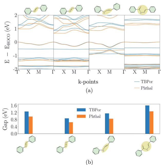
Fig. 3 (a) Electronic band-structures and (b) electronic band-gaps for the partially conjugated COFs. The different colors refer to the different cores, blue for TBPor and orange for Phthal-based COFs, respectively.
