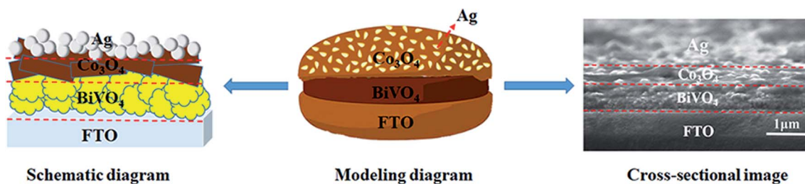
Fig. 1 Schematic diagram, modeling diagram and cross-sectional image of triadic Ag/Co 3 O 4 /BiVO 4 photoanode.
