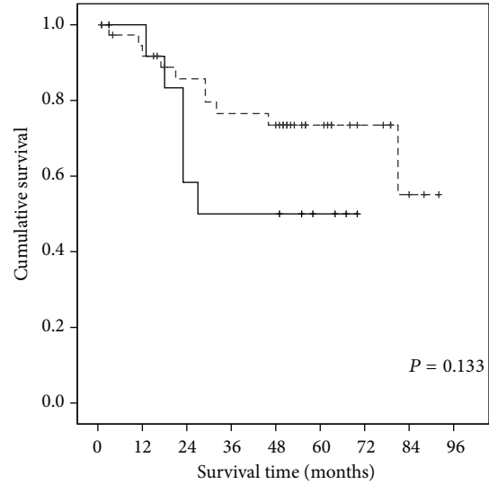
VEGF-A median - - - Low expression - - - Low expression censored — High expression — High expression censored
