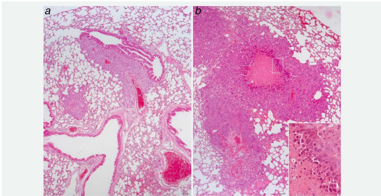
Figure 4. HE stained sections of the lungs of a NSG female mouse injected with (b) NMuMG cells cultured in the presence of \text{AlCl}_3 100 \mu\text{M} for 6 months or (a) NMuMG cells incubated for 6 months in the presence of a 1/1,000 dilution of \text{H}_2\text{O} . The mice were from the same experiment described in Figure 3. In (b), the inset shows necrotic cells. Bar in a and b = 50 \mu\text{m} .
