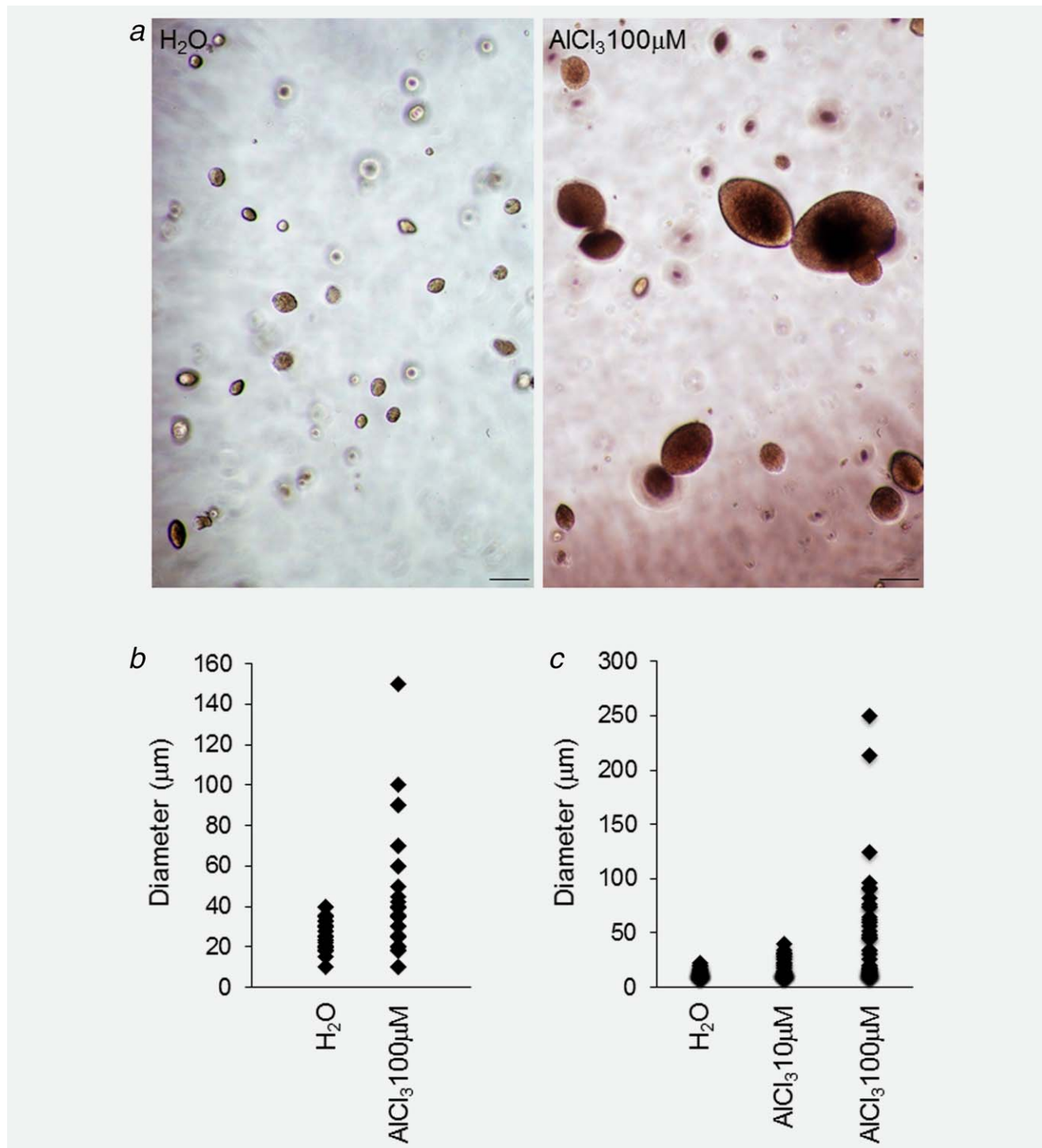
Figure 2. AlCl 3 transforms NMuMG cells in vitro . (a) NMuMG cells cultured for 4 months in the presence of AlCl 3 100 μM or the equivalent volume of H 2 O as control were resuspended in agarose gels at the density of 2 \times 10^4 cells/ml and grown for 14 days in the presence of complete culture medium. AlCl 3 was not added to the soft agar assay. Bar = 100 μm. (b) The growth in agarose gels was quantified by measuring the diameter of the structures (single cells or multicellular colonies) formed after 14 days. At least 50 randomly selected structures (single cells or multicellular colonies) from two independent experiments/condition were measured. p AlCl 3 versus H 2 O = 6.71E-04 (two-tailed t -test). (c) The graph shows the growth in agarose of NMuMG cells from a different source (ATCC), cultured for 7 months in the presence of AlCl 3 10 μM, AlCl 3 100 μM or the equivalent volume of H 2 O as control, as indicated. The soft agar assay was as described in a, b. p AlCl 3 10 μM versus H 2 O = 0.02; p AlCl 3 100 μM versus H 2 O = 2.79E-05 (two-tailed t -test). [Color figure can be viewed at wileyonlinelibrary.com ]
