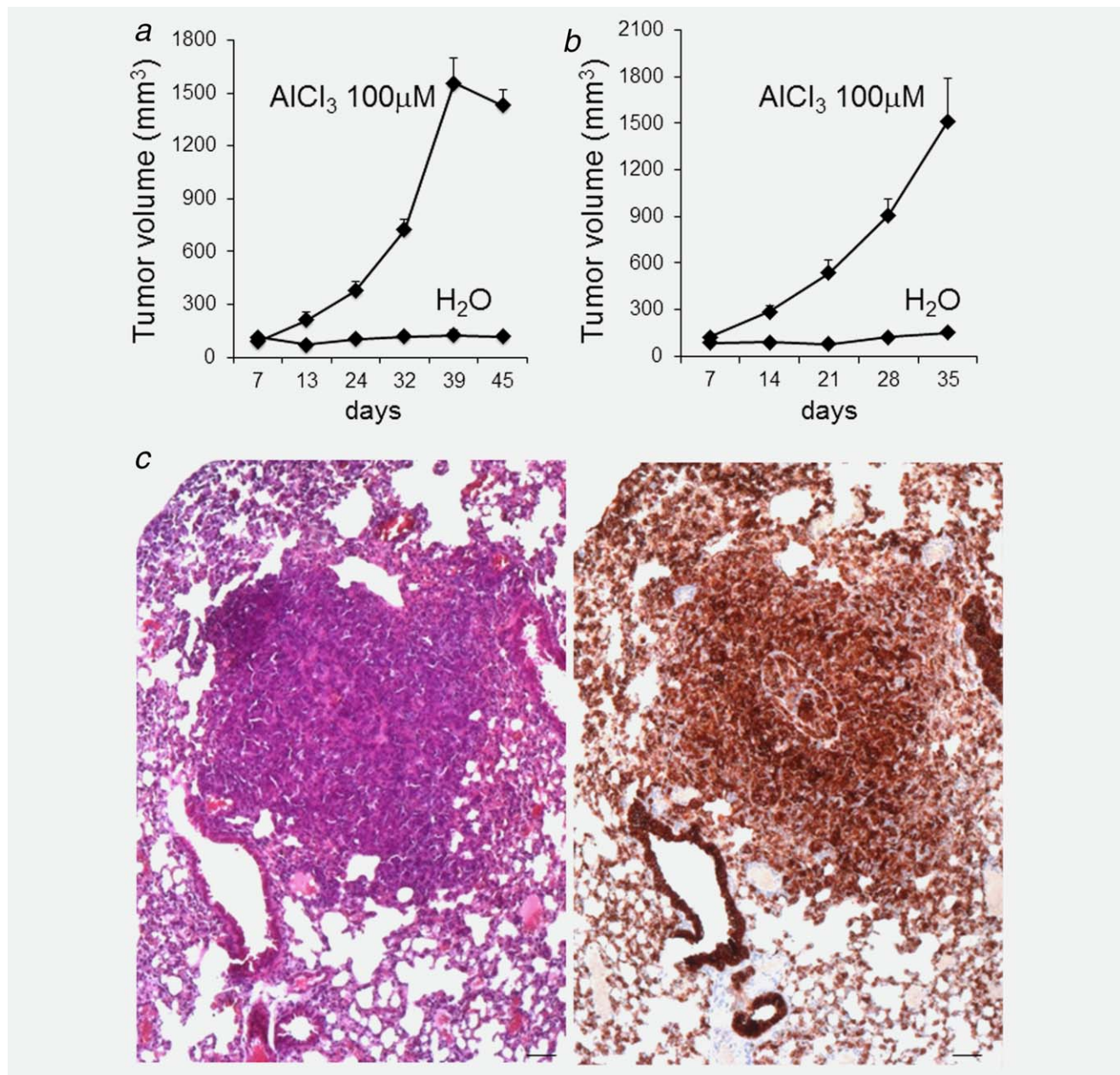
Figure 6. AlCl 3 promotes tumorigenesis and metastasis in NMuMG cells injected subcutaneously into NOD SCID and nude mice. (a) Five million NMuMG cells cultured for 8 months in the presence of AlCl 3 100 μM or the equivalent volume of H 2 O as control were resuspended in 200 μl of Matrigel and injected subcutaneously into the flank of 6-week-old NOD SCID female mice. Five mice/condition were used. Cell growth at the site of injection was measured with a caliper. The graph shows the volume ± SEM of such growth (calculated according to the formula V (\text{mm}^3) = d^2 (\text{mm}^2) \times D (\text{mm})/2 , where d and D are the smallest and largest tumor diameters, respectively) at the indicated number of days after injection. Tumor incidence was 100% (all the mice injected with AlCl 3 -treated cells formed tumors). p values (two-tailed t -test) comparing the two experimental groups were as follows: 7 days: p = 0.37 ; 13 days: p = 0.02 ; 24 days: p = 0.001 ; 32, 39 and 45 days: p < 0.001 . (b) Five million NMuMG cells cultured for 8 months in the presence of AlCl 3 100 μM or the equivalent volume of H 2 O as control were resuspended in 200 μl of Matrigel and injected subcutaneously into the flank of 6-week-old Swiss nude female mice. Five mice were used for AlCl 3 -treated cells, and four mice for control cells (the fifth mouse planned to be injected with control cells died during anesthesia at the time of injection). Cell growth at the site of injection was measured with a caliper. The graph shows the volume ± SEM of such growth (calculated according to the formula V (\text{mm}^3) = d^2 (\text{mm}^2) \times D (\text{mm})/2 , where d and D are the smallest and largest tumor diameters, respectively) at the indicated number of days after injection. Tumor incidence was 100% (all the mice injected with AlCl 3 -treated cells formed tumors). p values comparing the two experimental groups were as follows: 7 days: p = 0.11 ; 14 days: p = 0.0049 ; 21 days: p = 0.0017 ; 28 and 35 days: p < 0.003 (two-tailed t -test). (c) HE stained section (left) or cytokeratin 19 immunohistochemistry on an adjacent section (right) showing a lung metastasis in a Swiss nude mouse injected with AlCl 3 -treated NMuMG cells. Bar = 50 μm.
