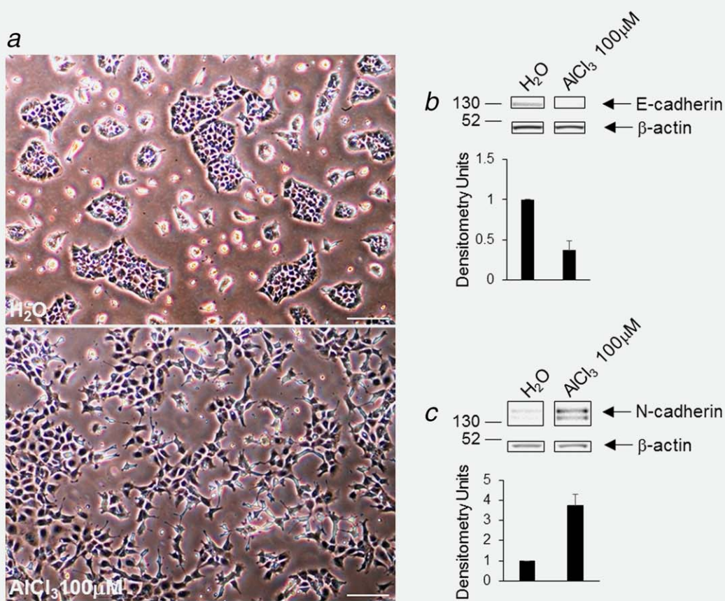
Figure 1. (a) Phase contrast view of NMuMG cells incubated for 4 months in the presence of AlCl 3 100 μM (bottom) or the same volume (1/1,000) of solvent (H 2 O) alone as a control (top). AlCl 3 or H 2 O were renewed twice a week with fresh culture medium. Bar = 100 μm. (b) Approximately 80% confluent NMuMG cells cultured for 6 months in the presence of AlCl 3 100 μM, or of the same dilution—1/1,000—of solvent (H 2 O) alone as a control were analysed for the expression of E-cadherin, or β-actin as a loading control, by Western Blotting. One representative gel (out of 6) is shown. The bands presented were from the same gel. The graph shows the mean values for E-cadherin expression, obtained in densitometric analysis, ± SEM, from six experiments, normalized with respect to β-actin levels. Control (H 2 O) was set to 1. p H 2 O versus AlCl 3 100 μM = 0.00038 (two-tailed t -test). (c) Same experiment as in (b), except that (i) cells were approximately 50% confluent; (ii) analysis was for N-cadherin; (iii) the number of experiments was 4; (iv) p H 2 O versus AlCl 3 100 μM = 0.0023 (two-tailed t -test). [Color figure can be viewed at wileyonlinelibrary.com ]
