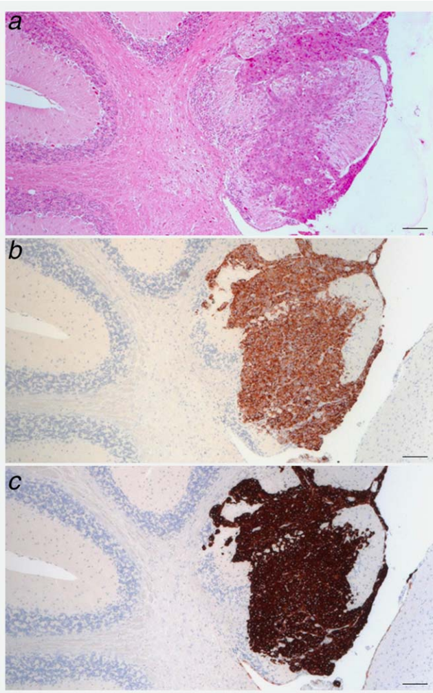
Figure 5. \text{AlCl}_3 promotes tumorigenesis and brain metastasis in NMuMG cells injected subcutaneously into NSG mice. (a) HE stained sections of the cerebellum of a NSG female mouse injected with NMuMG cells cultured in the presence of \text{AlCl}_3 100 \mu\text{M} for 6 months. The mouse was from the same experiment described in Figure 3. (b) Cytokeratin 7 or (c) cytokeratin 19 immunohistochemistry on adjacent sections. Bar in a, b, c = 50 \mu\text{m} .
