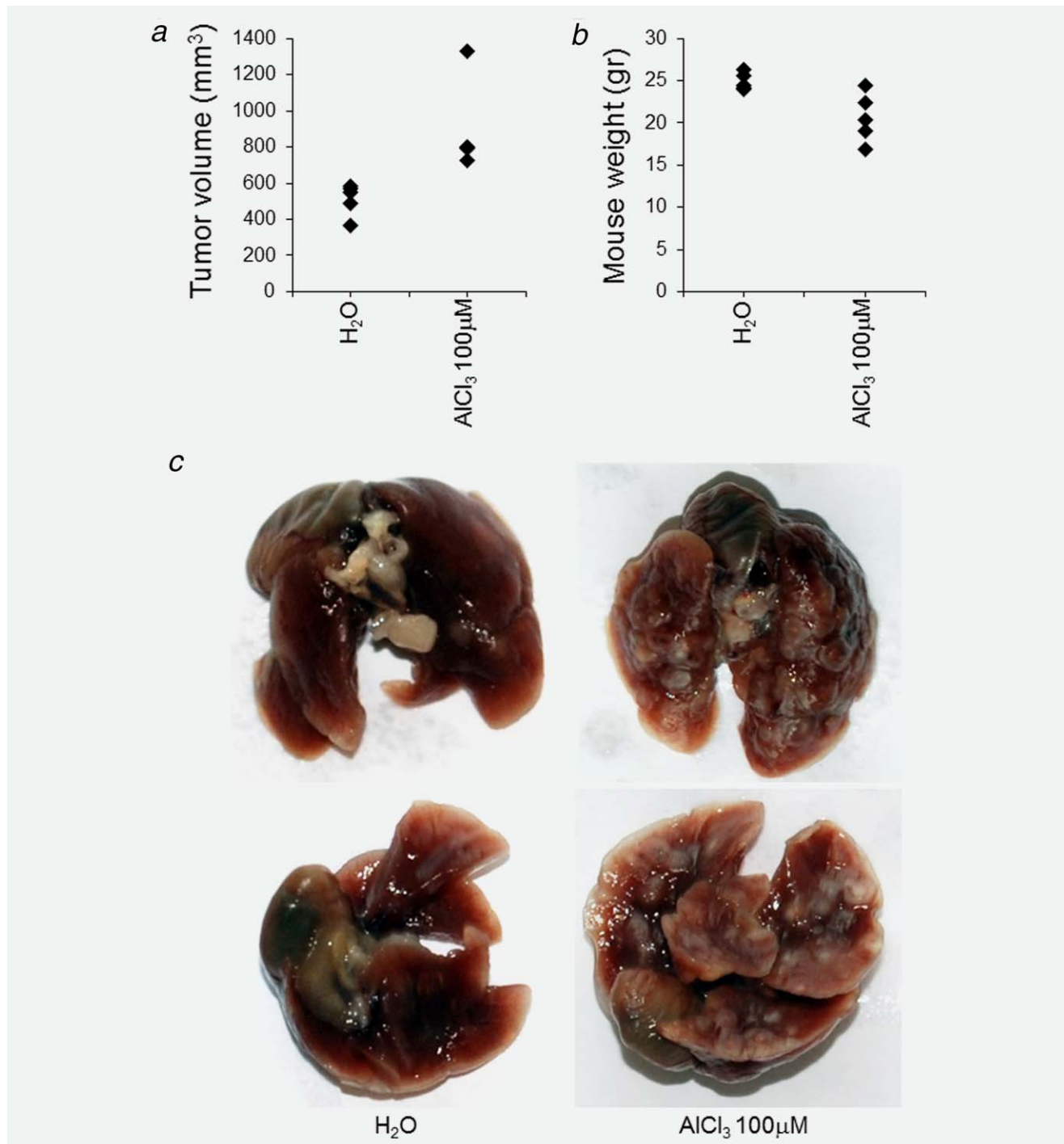
Figure 3. AlCl 3 promotes tumorigenesis and lung metastasis in NMuMG cells injected subcutaneously into NSG mice. Five million NMuMG cells cultured for 6 months in the presence of AlCl 3 100 µM or the equivalent volume of H 2 O as control were resuspended in 200 µl of Matrigel and injected subcutaneously into the flank of 6-week-old NSG female mice. Five mice/condition were used. The mice were sacrificed 6 weeks after injection. The graphs show (a) the volume of each tumor (calculated according to the formula 4/3\pi \times a \times b \times c , with a , b , c corresponding each to 1/2 of the three axis of the tumor, approximated to an ellipsoid, respectively) or (b) the weight of each mouse at the time of sacrifice. Tumor incidence was 100% (all the mice formed tumors). Statistics were as follows. For tumor volume, H 2 O versus AlCl 3 100 µM: p = 0.01 , two-tailed t -test. For mouse weight, H 2 O versus AlCl 3 100 µM: p = 0.01 , two-tailed t -test. (c) Macroscopic apical view (upper panel) or ventral view (lower panel) of the lungs of a NSG female mouse injected with AlCl 3 -treated NMuMG cells or H 2 O-treated NMuMG cells, as indicated, at the time of sacrifice.
