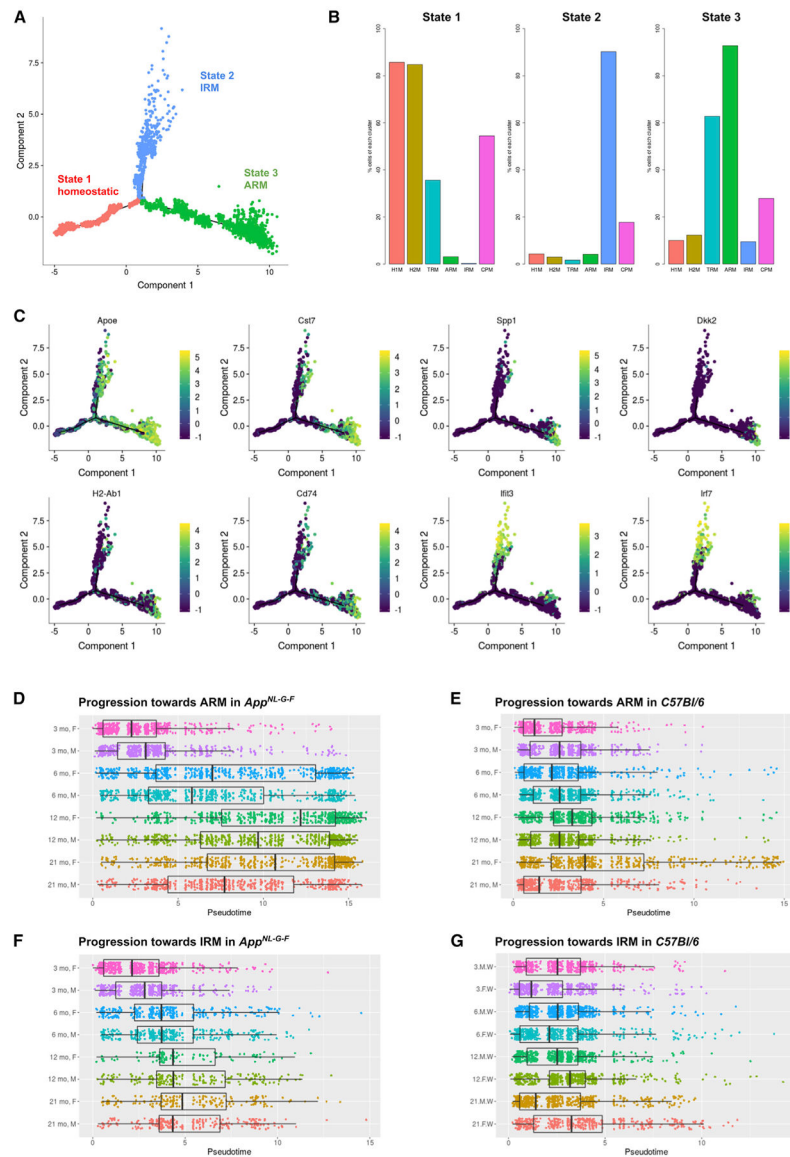
Figure 2. Microglia Diversify into Two Cell State Branches during Response to \beta -amyloid Plaques
