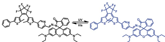
Scheme 1 Photochromism of diarylethene 1o .
