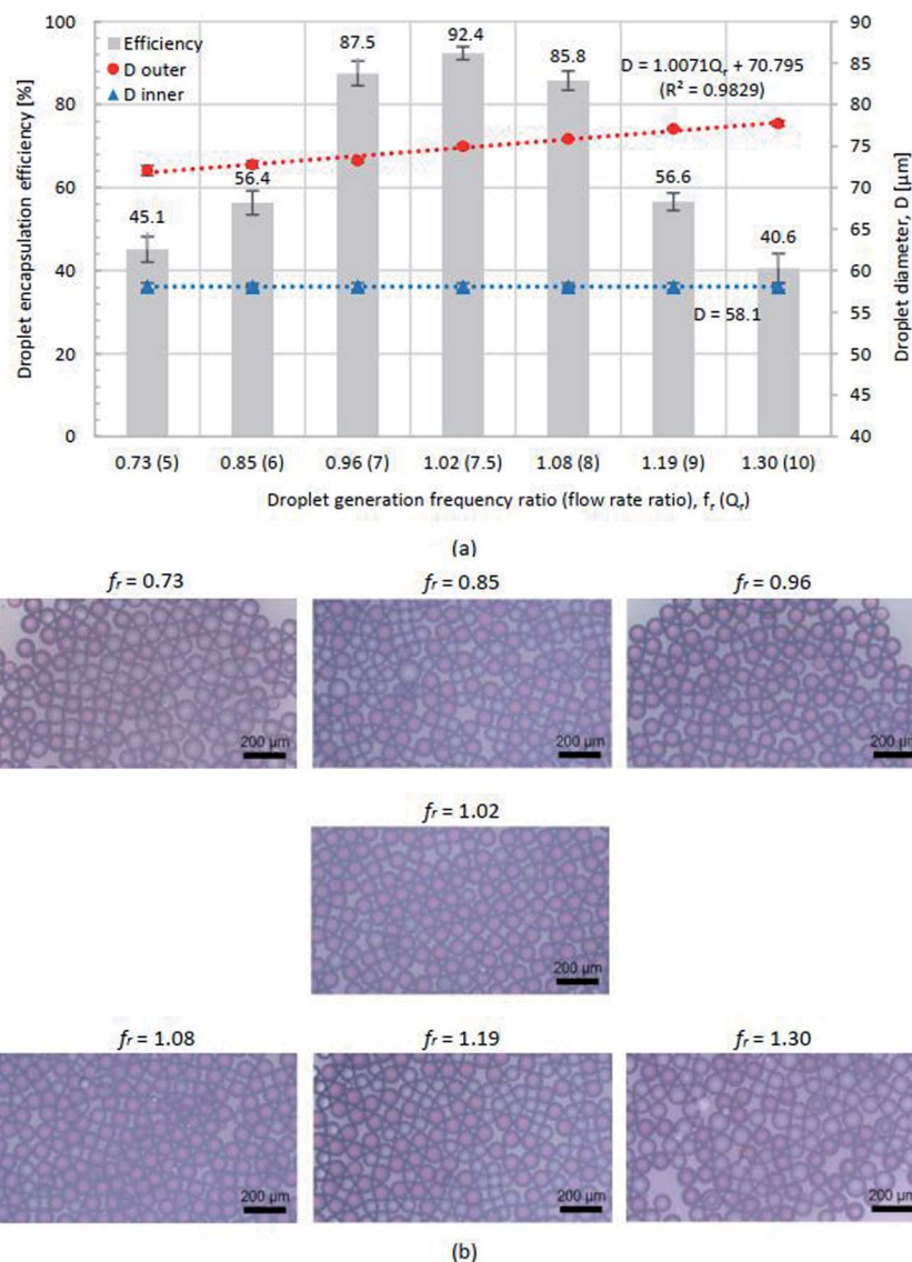
Fig. 7 (a) Droplet encapsulation efficiency (primary vertical axis) and droplet diameter (secondary vertical axis) and (b) images of water-in-oil-in-water droplets at f_r = 0.73 – 1.30 .
