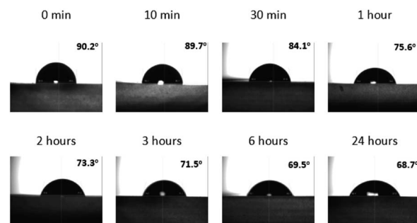
Fig. 4 Water contact angles of the WT1 sample after the hydrophilic surface treatment within 24 hours.
