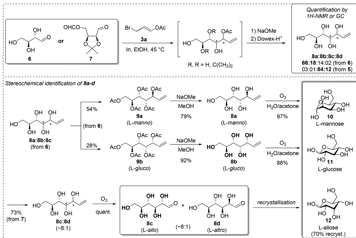
3,4- syn -selectivity (L-erythrose) based on a Cram-chelate model
