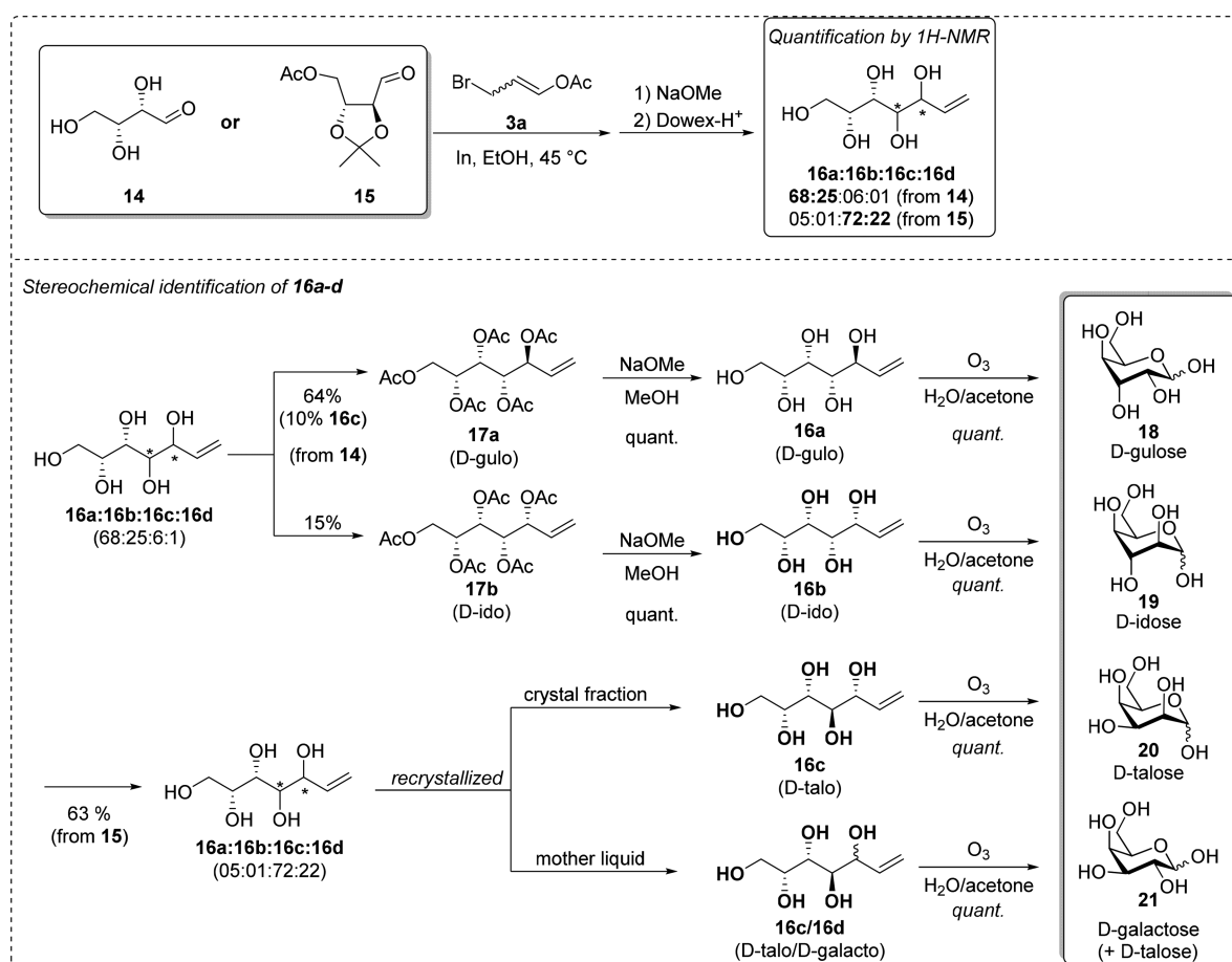
Scheme 3. Facial Diastereodivergence in the Indium Mediated Addition of 3a to Unprotected (14) and Protected (15) D-Threose (15)
