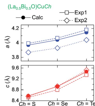
Fig. 2 Trend of lattice parameters of for (\text{La}_{0.5}\text{Bi}_{0.5}\text{O})\text{CuCh} (Ch = S, Se, Te) systems different Ch from calculation (Calc) and experiments of (\text{LaO})\text{CuCh} (Exp 1 ) and (\text{BiO})\text{CuCh} (Exp 2 ).
