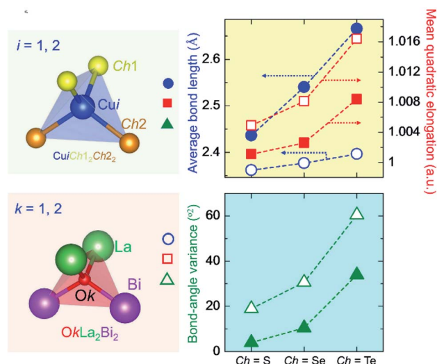
Fig. 3 Cu_iCh_2Ch_2 ( i = 1, 2 ) (top left panel) and OkLa_2Bi_2 ( k = 1, 2 ) tetrahedra (bottom left panel) in (La_{0.5}Bi_{0.5}O)CuCh ( Ch = S, Se, Te ) systems. The right panels present average bond length and local-symmetry distortion parameters (mean quadratic elongation and bond-angle variance) of both tetrahedra. Filled and unfilled shapes (circle, square, and triangle) denote those of Cu_iCh_2Ch_2 and OkLa_2Bi_2 tetrahedra, respectively.
