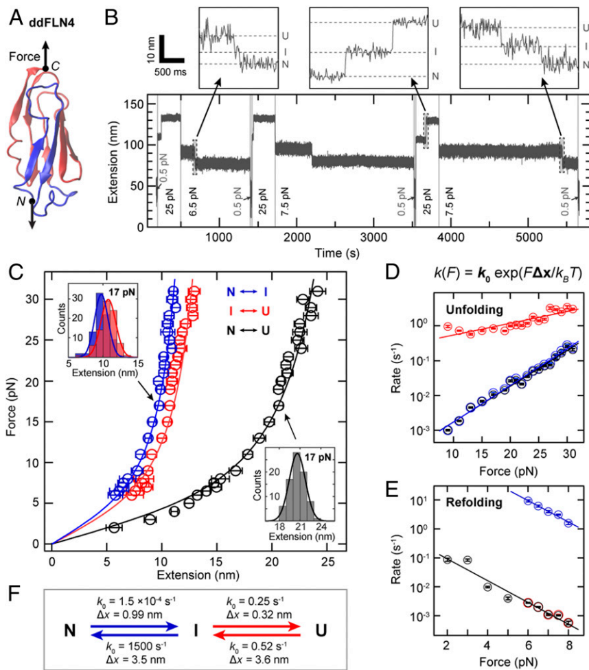
Fig. 2. Three-state folding and unfolding of ddFLN4 at constant force. (A) Structure of ddFLN4 [Protein Data Bank ID code 1K5R (83), rendered using VMD (84)], with strands A and B rendered in blue and strands C-G forming the structured portion of the intermediate state, in red. Arrows indicate the direction of force acting on ddFLN4's termini during MT experiments. (B) Extension vs. time trace of a ddFLN4 tether subjected to alternating intervals of high force (here 25 pN) allowing for ddFLN4 unfolding, intermediate force (here 6.5 or 7.5 pN) allowing for direct observation of refolding, and low force (0.5 pN) to ensure refolding before the next cycle. Unfolding and refolding of ddFLN4 via the mandatory intermediate state are observed as upward or downward double steps in the traces, respectively. Dashed lines in B , Insets indicate extension levels corresponding to the native (N), intermediate (I), and unfolded (U) states, respectively. (C) Force-extension profiles of ddFLN4 for the transitions N \rightarrow I (blue) and I \rightarrow U (red) and for full (un)folding N \rightarrow U (black). Data points are obtained by Gaussian fits to step extension histograms ( C , Insets ) at each constant force. Data points above 8 pN are from unfolding (based on 68–131 events obtained from 27–36 independent tethers), and data points up to 8 pN from refolding (54–159 events from 26–39 independent tethers). Error bars correspond to the full width at half maximum (FWHM) of Gaussian fits, divided by the square root of counts. Lines are fits of the WLC model. (D) Rates of unfolding at different constant forces for the 3 transitions. Color code is as in C . Error bars correspond to 95% CIs of exponential fits to the fraction of observed events as a function of time ( Materials and Methods and SI Appendix , Fig. S8). Lines are fits of a single-barrier kinetic model. (E) Rates of refolding at different constant forces. Color code, error bars, and fits are analogous to D . (F) Fitted rates at zero force k_0 and distances to the transition state \Delta x for the unfolding and refolding transitions as determined from the fits of a single-barrier kinetic model shown in D and E .
