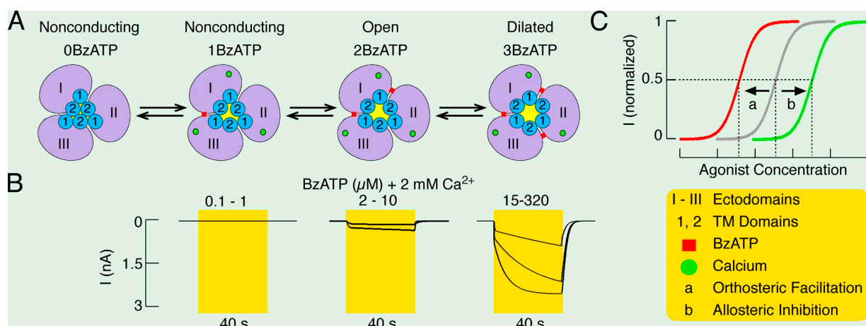
Figure 10. Orthosteric (BzATP) facilitation and allosteric (Ca 2+ ) inhibition of P2X7R. (A) In resting conditions (no agonist bound), the naive P2X7R is a symmetrical trimer, with three binding sites having equal and high affinity for orthosteric agonists, and is closed. The occupation of one binding site by agonist does not open the pore but leads to the loss of symmetry and an assumed reduction in the affinity of the two remaining binding sites as a result of a conformational change. When a second site is occupied, the affinity of the remaining binding site is further reduced, but the channel opens in a low conductance state. When three binding sites are occupied, however, symmetry is restored, and the binding rates revert to those of a naked receptor, allowing the pore to gradually dilate to a high conductance state and to sensitize. (B) The naive receptor in the open state generates monophasic currents with peak amplitude determined by BzATP concentration. The naive receptor at high BzATP concentration dilates and generates high amplitude biphasic currents. (C) Dependence of the peak current amplitude, measured 40 s after agonist application, on orthosteric and allosteric agonist concentrations. Gray trace, concentration dependence on BzATP of the peak current response of naive receptors in the presence of physiological bath Ca 2+ concentration. Red trace, concentration dependence on BzATP of the peak current response of sensitized receptors, termed orthosteric facilitation, in the presence of physiological Ca 2+ concentration. Green trace, concentration dependence on BzATP of the peak current response of naive receptors in the presence of elevated bath Ca 2+ . For details on orthosteric facilitation, see Yan et al. (2010). Experiments presented in this manuscript show that the rightward shift in the potency of agonist to activate P2X7R reflects allosteric inhibition of the receptor by this cation.
