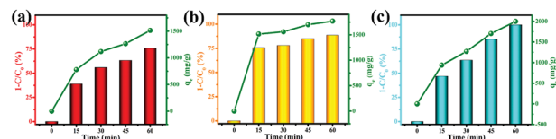
Fig. 7 Toxic ion adsorption experiments for (a) \text{Co}^{2+} , (b) \text{Cu}^{2+} , and (c) \text{Ni}^{2+} on MgO nanoparticles.
