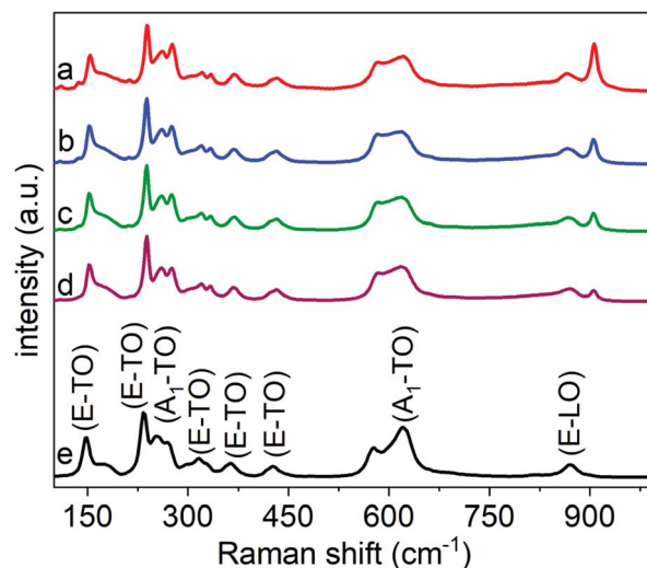
Fig. 5 Raman spectra for a series of \text{LiNbO}_3 particles, which were each calcined at 600^\circ\text{C} after their preparation by hydrothermal synthesis for: (a) 24 h; (b) 48 h; (c) 72 h; and (d) 96 h. (e) A Raman spectrum of a commercial \text{LiNbO}_3 powder included for comparison to the calcined products.
