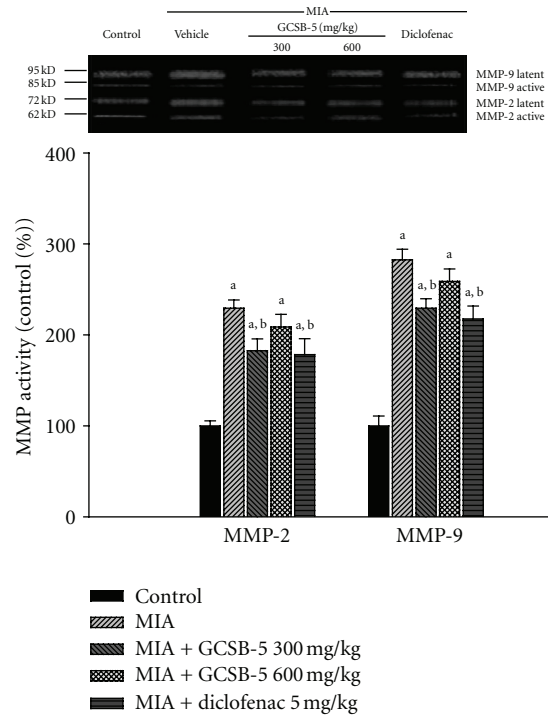
FIGURE 3: Activities of MMP-2 (Gelatinase A) and MMP-9 (Gelatinase B) assessed by zymography in knee joint cartilages obtained 28 days after MIA injection. The latent and active amounts of gelatinase were combined to give a total value for each gelatinase. Each value represents the mean \pm S.E.M. from 6 rats per group. a Significantly different ( P < 0.01 ) from control. b Significantly different ( P < 0.05 ) from vehicle-treated MIA.
