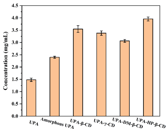
Fig. 7 Solubility histograms of crystalline UPA, amorphous UPA, and UPA-CD in artificial gastric juice at pH = 2 (mean \pm SD, n = 3 ).
