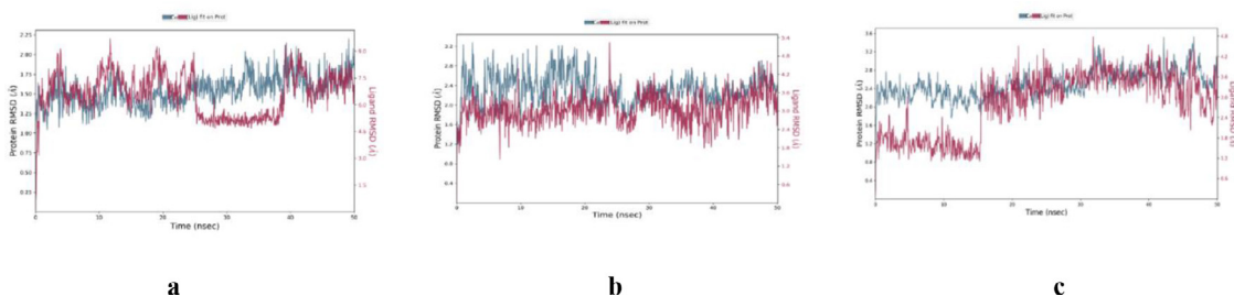
Fig. 8. RMSD plots of the C \alpha atoms of protein and the ligand with time: a) 8a-Mpro, b) 8b-PLpro, c) 9a-ACE2-S1'.
