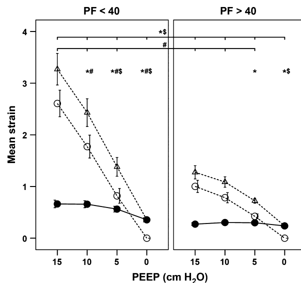
Fig. 4. Changes in strain during a decremental PEEP trial for patients with normal oxygenation or impaired oxygenation within the CABG group. Data are shown as mean \pm SE. Strain is calculated for coronary artery bypass graft (CABG) patients with a PaO 2 /FiO 2 ratio smaller or larger than 40 kPa. Open triangles: global stress or strain; open circles: static stress or strain (PEEP); closed circles: dynamic stress or strain (tidal volume); dashed lines: interpolation lines. All differences are considered to be significant if P < 0.05 . *Significant differences in global strain; #Significant differences in static strain; $Significant differences in dynamic strain.
