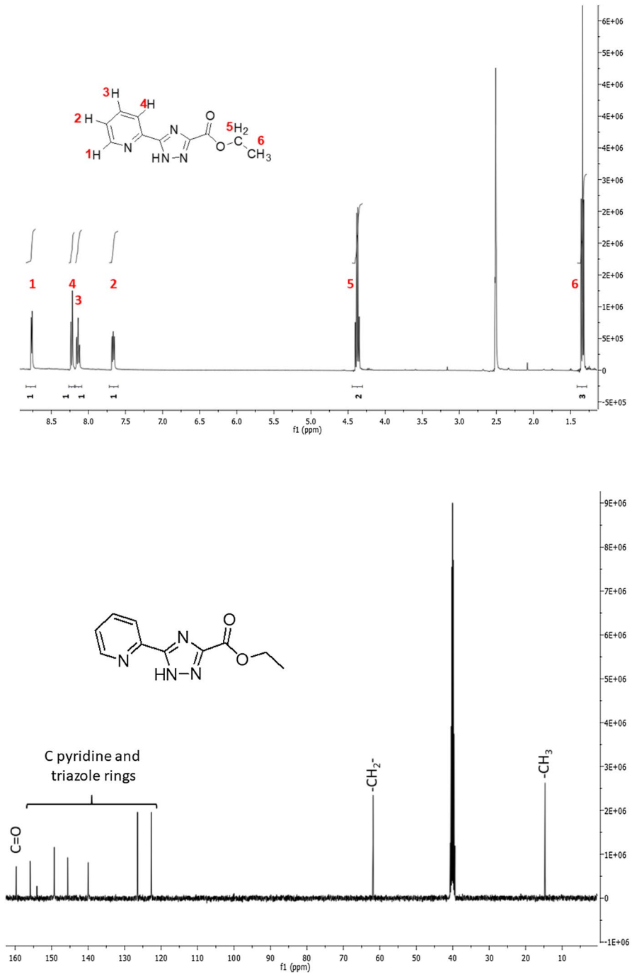
Fig. 1 ^{13}\text{C} and ^1\text{H} NMR spectra of 5-Pyridin-2-yl-1H-[1,2,4]triazole-3-carboxylic acid ethyl ester
