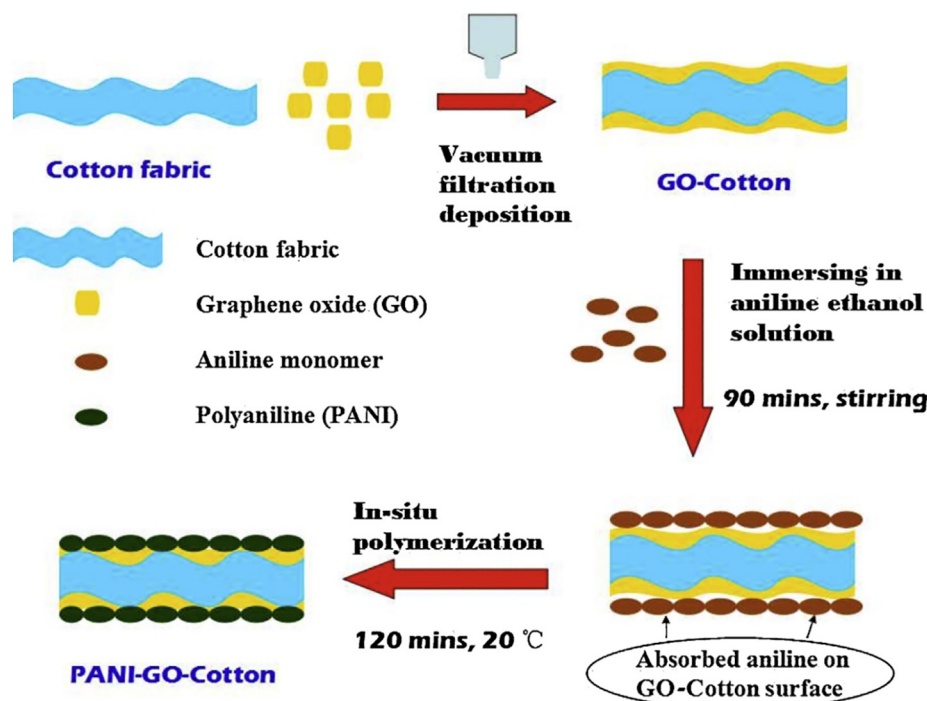
Fig. 3. Preparation procedure of PANI-GO-cotton fabric [34]. Reprinted with permission from Elsevier.
