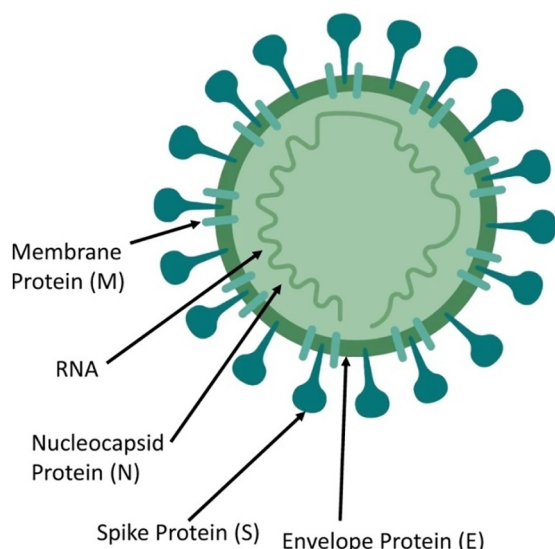
Fig. 1. Main structure of Corona viruses [4]. Reprinted under the terms of the Creative Commons CC BY license.
