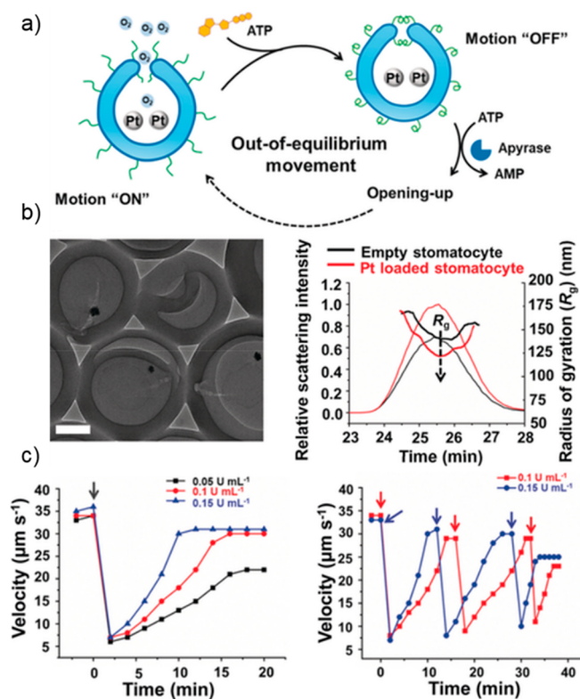
Figure 7. (a) Schematic of the transient deactivation and activation of a stomatocyte nanosystem mediated by ATP. (b) Polylysine (PLL)-modified stomatocytes loaded with Pt nanoparticles (PtNP) are characterized by TEM and asymmetric flow field-flow fractionation (AF4). Scale bar = 100 nm. (c) Velocity of the PtNP-loaded PLL-stomatocyte nanomotors as a function of time upon the addition of ATP in the presence of different concentrations of apyrase. Three cycles of the adaptive nanomotor system upon the repeated addition of ATP. The arrows indicate the addition of ATP. Reproduced from ref 102 with permission from John Wiley and Sons. Copyright 2019 Wiley-VCH Verlag GmbH & Co. KGaA, Weinheim.
