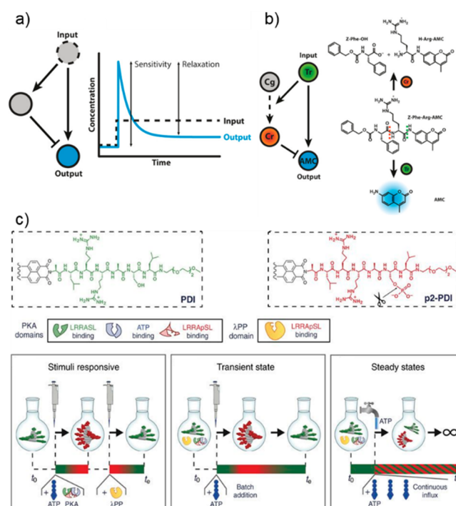
Figure 6. (a) Adaptive enzymatic reaction network with an incoherent feed-forward loop, in which the output is positively controlled in a direct manner but negatively controlled in an indirect manner, and a typical shape of an adaptive or pulse-like response (blue line) in response to a persistent input (dashed black line). The sensitivity is a measure of the strength of the response relative to the input. Relaxation compares the steady-state response to the maximum response. (b) A typical example of an adaptive enzymatic reaction network, inspired by the feed-forward loop network motif, with trypsinase producing a persistent input. (c) Nonequilibrium steady states in supramolecular polymerization, in which the addition of ATP and Protein kinase A to a solution of a peryleneimide derivative results in diphosphorylation and subsequently a change in the structure and stereochemistry of the supramolecular polymer. The addition of protein phosphatase is needed to reset the polymer to its original nonphosphorylated state. The addition of ATP to a solution of the peryleneimide derivative, in the presence of both protein kinase A and protein phosphatase, leads to a transient change of the supramolecular structure. The supramolecular nonequilibrium system is kept in a dissipative steady state by continuous influx of ATP. (a, b) Reproduced from ref 119 with permission from John Wiley and Sons. Copyright 2018 Wiley-VCH Verlag GmbH & Co. KGaA, Weinheim. (c) Reproduced from ref 120 under Creative Commons Attribution https://creativecommons.org/licenses/by/4.0/ . Copyright 2017 A. Sorrenti et al.
