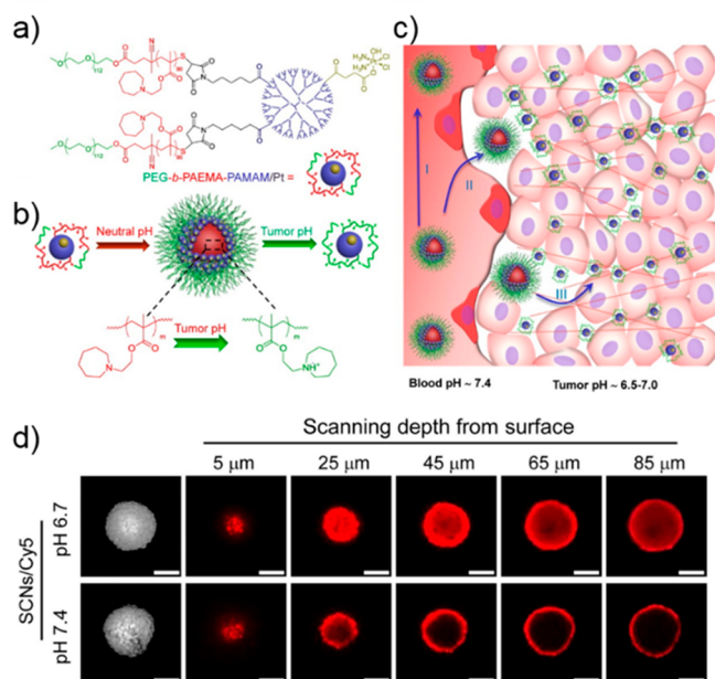
Figure 1. (a) Chemical structure of the transformable nanoparticles conjugated with Pt prodrug. (b) Mechanism displaying the pH-induced protonation of the hydrophobic block, resulting in a size switch behavior. (c) Illustration of the interactions of the transformable particles with cells and deeper penetration into tissue. (d) In vitro penetration of Cy5-labeled nanoparticles in a 3D tumor model, observed by confocal laser scanning microscopy (CLSM), indicating the effect of pH on penetration ability (scale bar = 100 μm). Figure reproduced with permission from ref 52. Copyright 2016 American Chemical Society.
