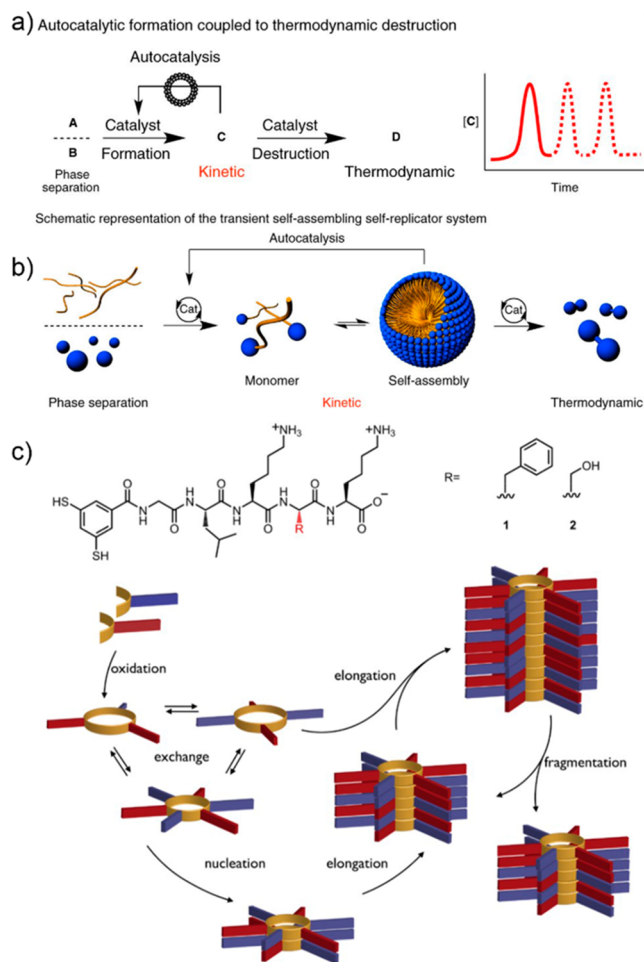
Figure 5. Transient self-assembling self-replicators and examples of autocatalysis. (a) An autocatalytic system based on phase separation, coupled to thermodynamic destruction, which in a closed experimental setup evolves toward thermodynamic equilibrium. (b) Schematic representation of a transient self-assembling self-replicator system. (c) Formation of a dynamic combinatorial library of macrocyclic disulfides by thiol oxidation of the building blocks 1 and 2 with two different peptide sequences, followed by disulfide exchange (only some of the possible combinations are shown). Mechanism of replication in a two-component system: the building blocks form an exchanging mixture of macrocycles of different sizes and building-block compositions via oxidation of thiols to give disulfide bonds and subsequent disulfide exchange. The hexamer macrocycles self-assemble into fibers as the peptide chains (arrows) form \beta -sheets through a nucleation–elongation mechanism. The fibers grow from their ends and break on mechanical agitation, which doubles the number of fiber ends that further promote the formation of self-replicating hexamer. (a, b) Reproduced from ref 111 under Creative Commons Attribution https://creativecommons.org/licenses/by/4.0/ . Copyright 2018 I. Colomer et al.
