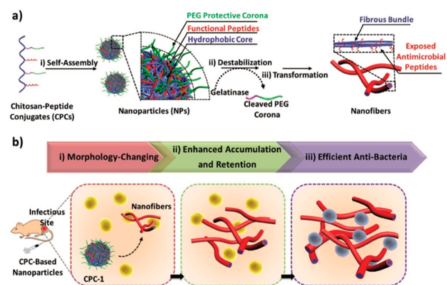
Figure 2. Illustration of the self-assembly of CPCs and the principle of enzyme-induced morphology transformation. (a) The CPCs self-assembled into nanoparticles with a pegylated protecting corona which was peeled off by gelatinase. Hydrogen bonding interactions between chitosans resulted in reorganized self-assembly into fibrous structures by the change of the ratio of the hydrophobic/hydrophilic parts. (b) CPC-based nanoparticles went through a morphology transformation as the gelatinase (produced by the bacteria at the infectious site) cleaved the peptide linker. Nanofibers with exposed antimicrobial peptide showed enhanced accumulation and retention which resulted in efficient antibacterial efficiency. Reproduced from ref 78 with permission from John Wiley and Sons. Copyright 2017 Wiley-VCH Verlag GmbH & Co. KGaA, Weinheim.
