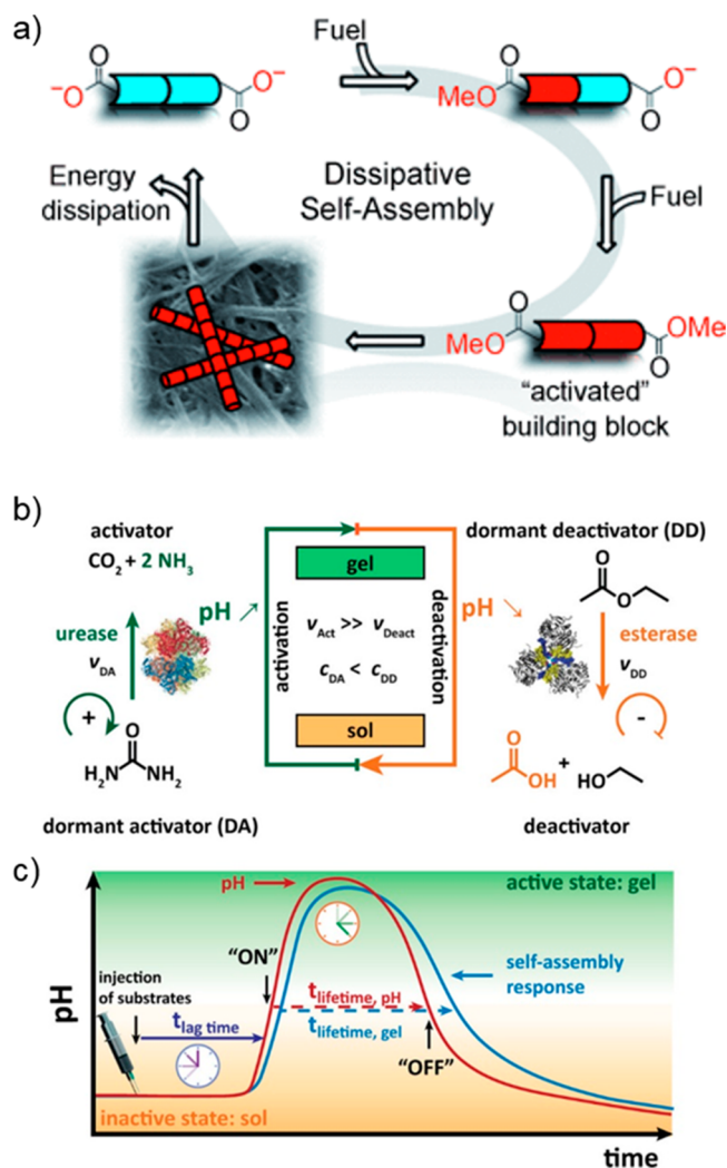
Figure 4. (a) Dissipative self-assembly process of a molecular gelator to form fibrillar networks from an activated building block, which is obtained from a synthetic gelator in a dissipative self-assembly process that is fueled by an alkylating agent. The system reverts to its thermodynamic equilibrium, when the available energy is depleted. (b) Biocatalytic temporal control of a self-regulating transient pH-state by kinetic balancing of two antagonistic feedback-controlled enzymatic pH reactions, in which a biocatalytic reaction network is used for internal pH modulation; the enzyme urease converts urea to the basic ammonia, a process that is amplified by autocatalytic positive feedback, while the antagonistic esterase transforms an ester to acid under negative feedback control. (c) Schematic of the transient alkaline pH-profile (red) with an initial lag time as produced by the biocatalytic reaction network in conjunction with the coupled self-assembly response (blue). Initially, the system is dormant and then becomes activated by simultaneous injection of the urea and the ester. Addition of an acidic buffer elongates the quasi-dormant period and implements an initial lag time to the system. (a) Reproduced from ref 100 with permission from John Wiley and Sons. Copyright 2010 Wiley-VCH Verlag GmbH & Co. KGaA, Weinheim. (b, c) Reproduced with permission from ref 101. Copyright 2017 American Chemical Society.
