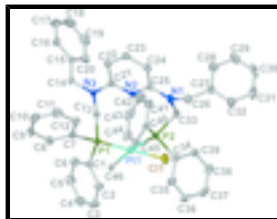
Fig. 1. The atom-numbering scheme of the title complex I. Displacement ellipsoids are drawn at the 30% probability level and H atoms are omitted for clarity.
