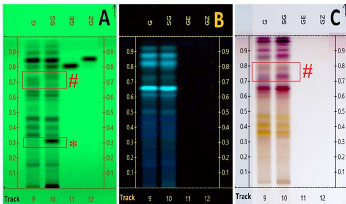
Fig. 1 Comparative HPTLC analysis of guggulu (G) and shodhita guggulu (SG) at 254 nm (A), 366 nm (B), and 514 nm (C) w.r.t. their marker compounds. Track 9: guggulu (G), track 10: shodhita guggulu
