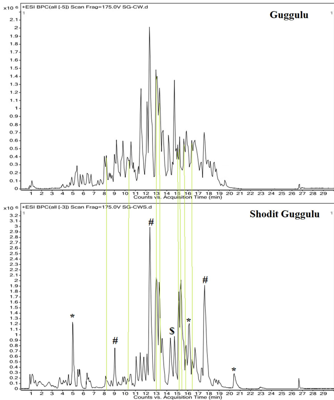
Fig. 2 Comparative LC–MS chromatograms of guggulu and shodhita guggulu ESI (+ve) mode; 5-(13'Z-nonadecenyl)resorcinol (Rt 8.31); 8 \beta -hydroxy-3,20-dioxopregn-4,6-diene (Rt 10.33); guggulsterone E (Rt 12.99); guggulsterone Z (Rt 13.28); guggulsterol I (Rt=15.19);
