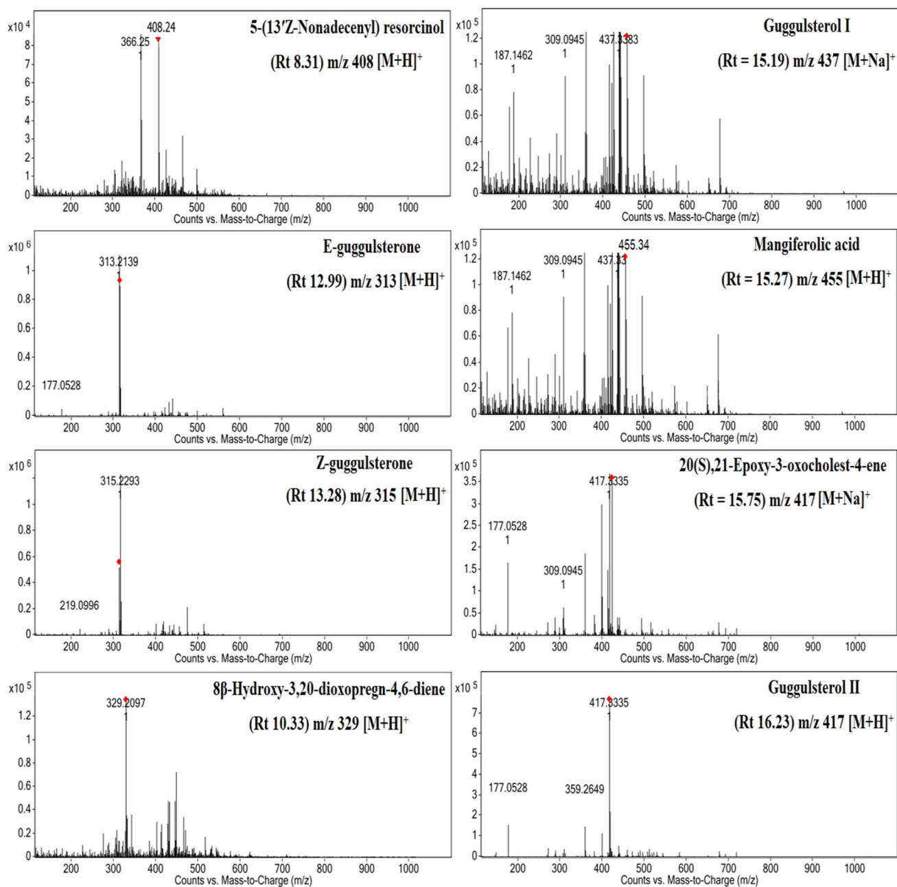
Fig. 3 Major fragmentations pattern of guggulu and shodhita guggulu observed in LC–MS ESI (+ve) mode study; 5-(13'Z-nonadecenyl) resorcinol (Rt 8.31); 8 \beta -hydroxy-3,20-dioxopregn-4,6-diene
