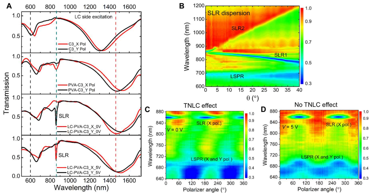
Fig. 2. Linear characteristics of the hybrid liquid crystal (LC)–threefold rotational symmetry (C3) metadvice. (A) Transmission spectra of the bare C3 metasurface, PVA-C3 sample, and LC-PVA-C3 sample for x - and y -polarized incident light, respectively. A strong nonlocal surface lattice resonance (SLR) mode at 860 nm wavelength is observed when x -polarized incident light interacts with the metasurface in LC-PVA-C3 sample. The effect of twisted nematic LC (TNLC) layer with applied voltage is clearly observed. No SLR mode is observed in the bare C3 metasurface. However, a very weak SLR mode is observed in PVA-C3 sample. (B) Angle-dependent SLR dispersion curves for LC-PVA-C3 sample in the nematic phase, where \theta is the angle in the yz plane. Polarization-dependent excitation of SLR mode with applied voltage (C) V = 0 V (TNLC effect) and (D) V = 5 V (no TNLC effect), respectively. LSPR, localized surface plasmon resonances.
