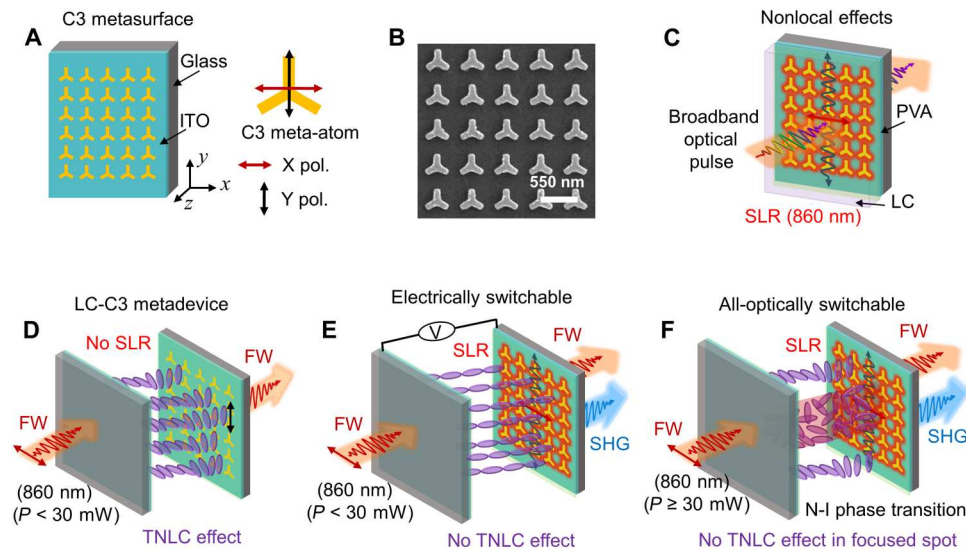
Fig. 1. Illustration of nonlocal effects in liquid crystal (LC)–threefold rotational symmetry (C3) metadvice. (A) Schematic of metasurface with C3 symmetry meta-atoms fabricated on indium tin oxide (ITO)–coated glass substrate. (B) Scanning electron micrograph of the fabricated metasurface before spin coating of the PVA layer. Scale bar, 550 nm. (C) Schematic view of excitation of x-polarized dependent nonlocal surface lattice resonance (SLR) mode (860 nm). (D) Schematic representation of the working principle of the twisted nematic LC (TNLC) layer. The TNLC layer rotates the polarization of incident x-polarized light by 90° and converts it to y-polarized light. Schematic representation of (E) electrical switching and (F) all-optical switching of second-harmonic generation (SHG) at SLR. The metadvice is excited at an SLR wavelength of 860 nm that generates SH signal when x-polarized light interacts with the metasurface. The N-I phase transition is observed at P = 30 mW. FW, fundamental wavelength.
