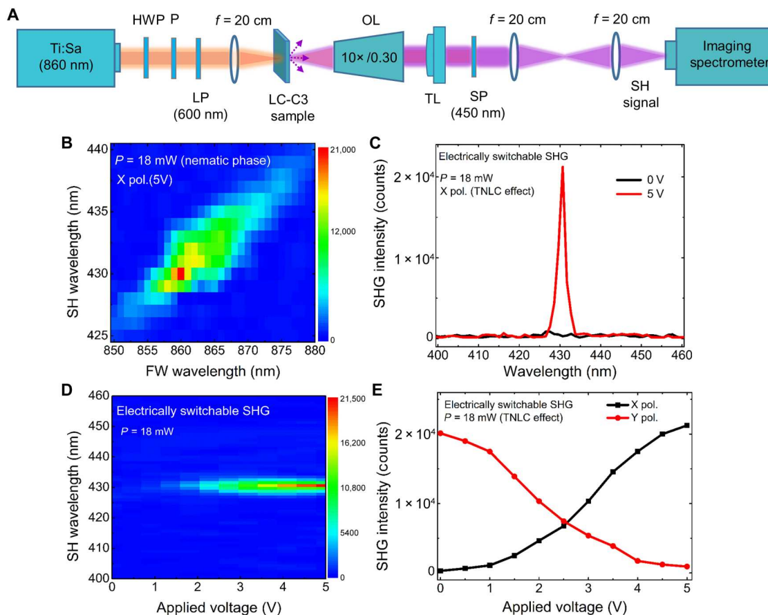
Fig. 3. Excitation and electrical tuning of nonlocal SH signal. (A) Schematic of the experimental setup that consist of a Ti:Sa light source, half-wave plate (HWP), polarizer (P), long-pass filter (LP), three focusing lenses ( f = 20 cm), liquid crystal (LC)–threefold rotational symmetry (C3) metadvice, objective lens (OL), tube lens (TL), short-pass filter (SP), and the imaging spectrometer. (B) Measurement of second-harmonic generation (SHG) excited at normal incidence for x-polarized fundamental wavelength (FW) with wavelength varying between 850 and 880 nm. The voltage on the cell is 5 V orienting the LCs in the z direction. It is clearly observed that the SH signal is strongly enhanced with narrow linewidth at the surface lattice resonance (SLR) wavelength (860 nm). (C) Electrical switching of the SHG at 0 and 5 V. (D) 2D plot for variation in SHG intensity with applied voltage 0 to 5 V. (E) Variation in SH signal with applied voltage when x- and y-polarized light excites. TNLC, twisted nematic LC.
