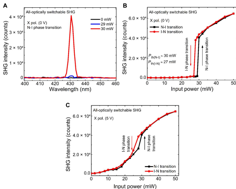
Fig. 4. All-optically switchable SH signal. (A) Measured second-harmonic (SH) signal for P = 29 mW and P = 30 mW, below and above threshold, respectively. (B) SH signal versus input power at 0 V for x-polarized incident light. At threshold power P = 30 mW, SH signal is abruptly enhanced because of optically induced phase transition. (C) SH signal versus input power at 5 V for x-polarized incident light. A slight step-like increment is observed near 30 mW at nematic-to-isotropic (N-I) phase transition. SHG, second-harmonic generation; I-N, isotropic-to-nematic.
