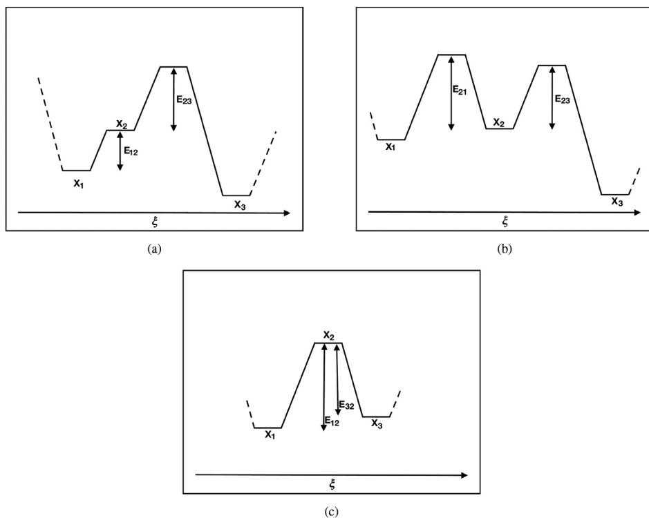
Fig. 8. Energy scheme representation of different reaction spots. (a) X_1 undergoes to a structural rearrangement, like a free rotation, before converting to X_3 ; (b) the conversion from X_1 to X_3 occurs through the formation of the X_2 intermediate; (c) a labile intermediate, X_2 , is a maximum along the reaction profile. X_i represents a given surface species, \xi is the reaction coordinate while E_{ij} is the energy barrier needing in the X_i \rightarrow X_j process.
