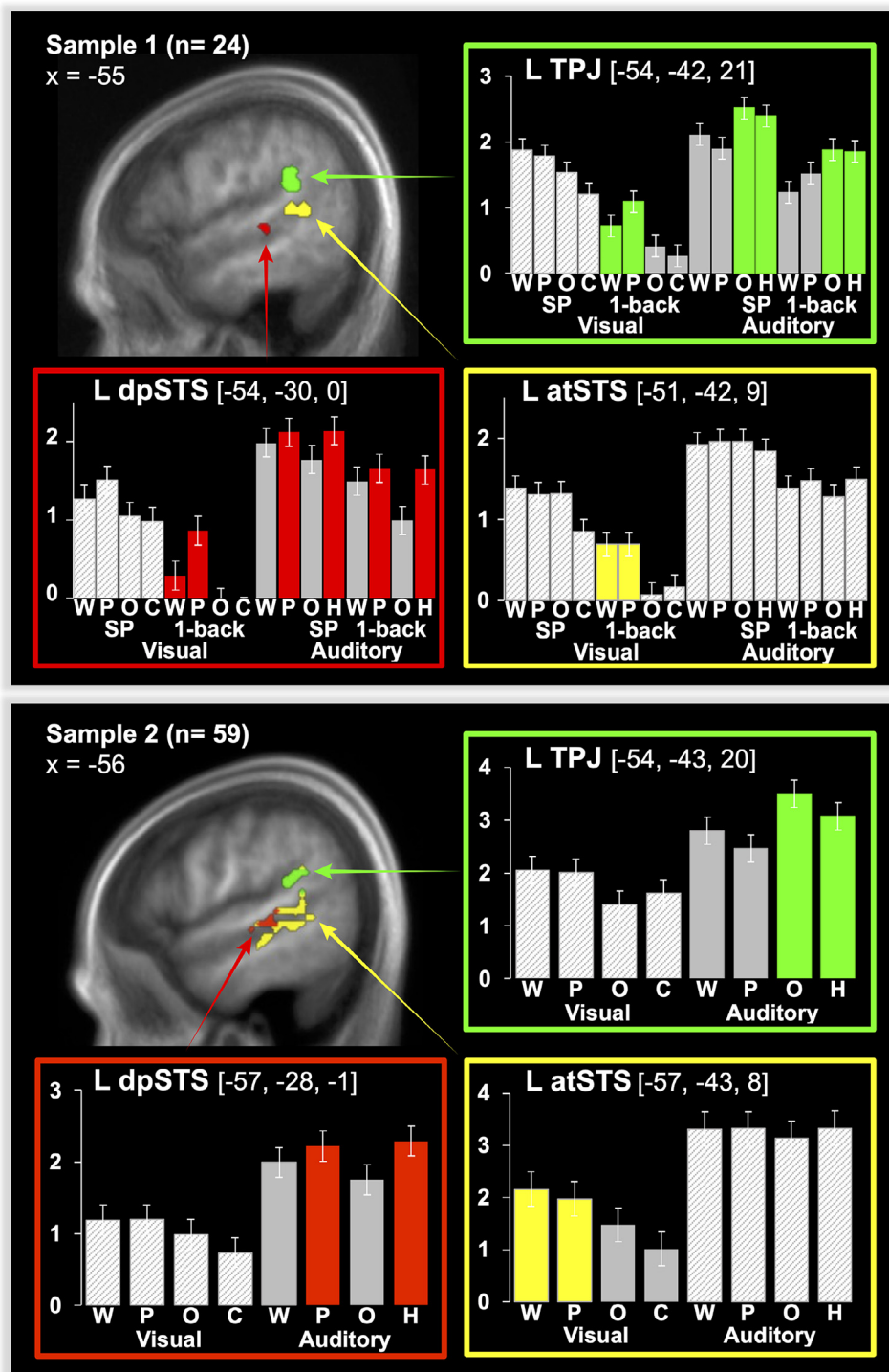
Fig. 3. Condition-specific responses in three left posterior superior temporal regions. The upper section shows the results from Sample 1. The lower section shows the results from Sample 2. For each sample, activation within the anatomical regions of interest (Fig. 1) are shown on the mean structural image for that sample. The three plots for each sample show the mean relative activation per condition (16 for Samples 1, 8 for Sample 2), with standard error bars. The coloured bars show conditions of interest (weighted +1 in the statistical contrast), the grey bars show the corresponding baseline conditions (weighted -1 in the statistical contrast) and the hashed bars show conditions that were not included in the statistical contrasts. Different colours (in both the plots and the brain image) distinguish different statistical contrasts in the auditory modality: green activation is higher for non-verbal than verbal auditory stimuli; red activation is higher for non-semantic than semantic auditory stimuli and yellow activation was not significantly different for verbal, non-verbal, semantic or non-semantic auditory stimuli. For Sample 1, each statistical contrast in the auditory modality was in conjunction with the effect of verbal more than non-verbal stimuli during visual 1-back matching. The verbal stimuli are words (W) and pseudowords (P). The non-verbal stimuli are objects (O), coloured patterns (C) and humming (H). The semantic stimuli are W & O. The non-semantic stimuli are P, C and H. SP = speech production tasks; 1-back = 1-back matching tasks. For Sample 1, peak effects were all significant at p < 0.05 FWE-corrected for multiple comparisons within the anatomical regions of interest (see Table 5A), and the extent of the effect is illustrated at a height-level threshold of p < 0.001 uncorrected. For Sample 2, the significance threshold was set at p < 0.05 uncorrected (Table 5C) but the effects were all significant with small volume correction at the peak co-ordinate for Sample 1 (see text). (For interpretation of the references to color in this figure legend, the reader is referred to the web version of this article.)
