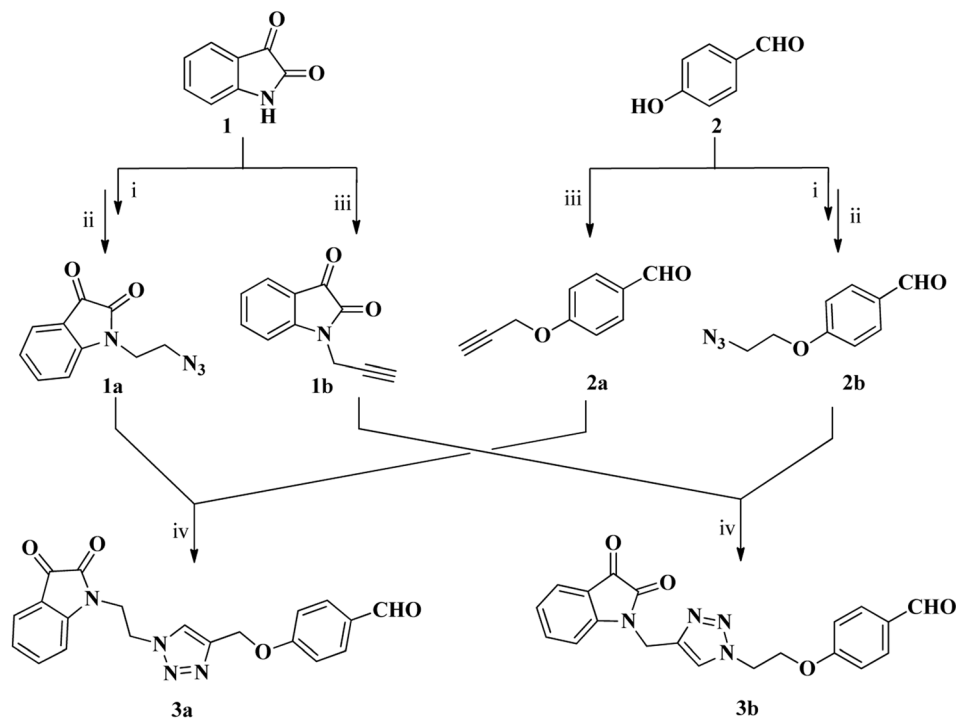
Scheme 1 Synthesis of isatin–triazole hybrids 3a and 3b ; reagents and conditions: (i) dibromoethane (2.1 eq.), DMF, \text{K}_2\text{CO}_3 (ii) \text{NaN}_3 (1.2 eq.), DMF (iii) propargyl bromide, DMF, \text{K}_2\text{CO}_3 (iv) \text{CuSO}_4 \cdot 5\text{H}_2\text{O} , sodium ascorbate, EtOH : \text{H}_2\text{O} (9 : 1), rt.
