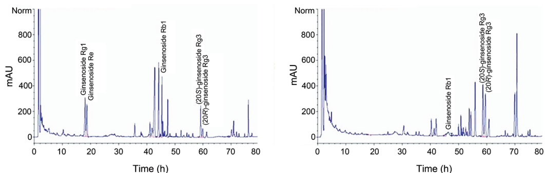
Fig. 2. HPLC fingerprints of fresh ginseng extract simmered for 3 and 24 h. The HPLC setup: Discovery HS C18 material (Supelco; 250×4.6 mm, 5 \mu m) at room temperature (25°C) with a sample injection volume of 20 \mu L (20 mg/mL); mobile phase: acetonitrile and water gradient.
