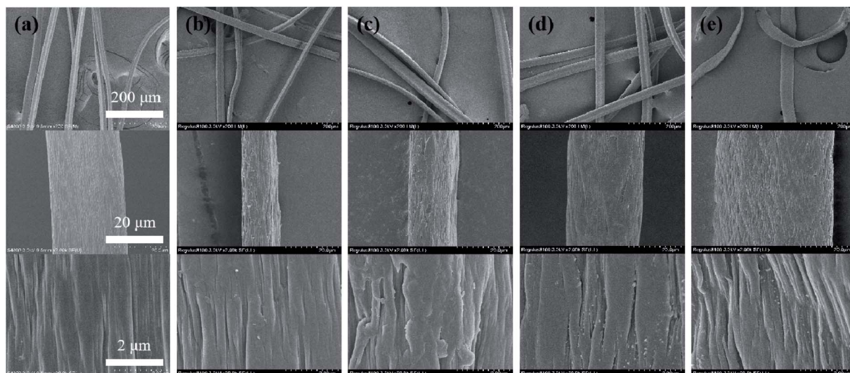
Fig. 4 The SEM images of (a) PANF, (b) PAN TA F, (c) PAN QA-C F, (d) PAN QA-C F-Ag(0) and (e) PAN QA-C F-Ag(0)-20. Top row 200 \times , middle row 2000 \times and bottom row 20 000 \times magnification.
