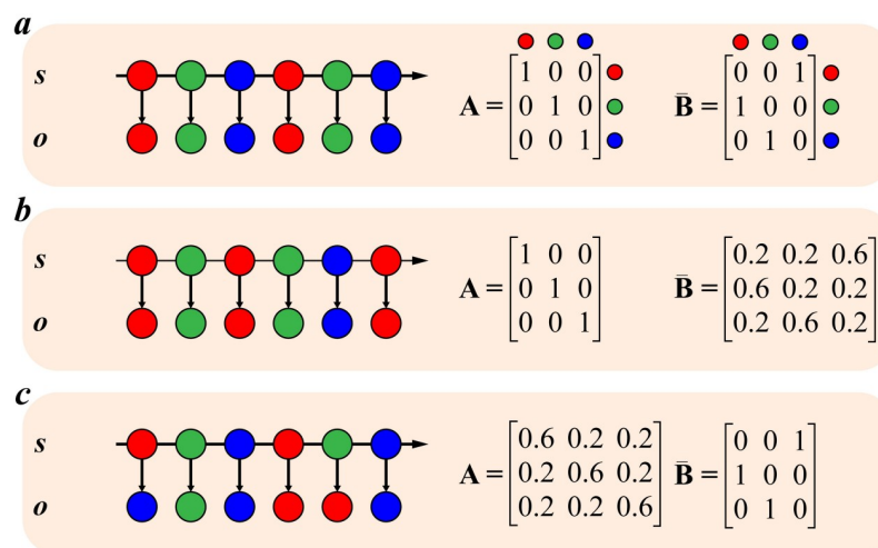
Fig 2. Sequences of outcomes emerging from random transition dynamics. Fig 2a shows the sequence of outcomes (o) produced by the sequence of states (s) when the transition matrices for both sequences are deterministic. Fig 2b shows the sequence of states, and outcomes those states generate, when the matrix defining the transitions between states ( B ) is not deterministic. Even though the transitions from states to outcomes are still deterministic, as in Fig 2a, the final sequence of outcomes is different. In Fig 2c we show the consequences of introducing randomness into the transitions (matrix A ) from states to events. The sequence of states remains the same as in Fig 2a, but the outcomes generated by each state are random, resulting in a different sequence of outcomes. Figs 2a and 2c demonstrate how randomness in the transition matrices can result in unpredictable sequences of outcomes.
