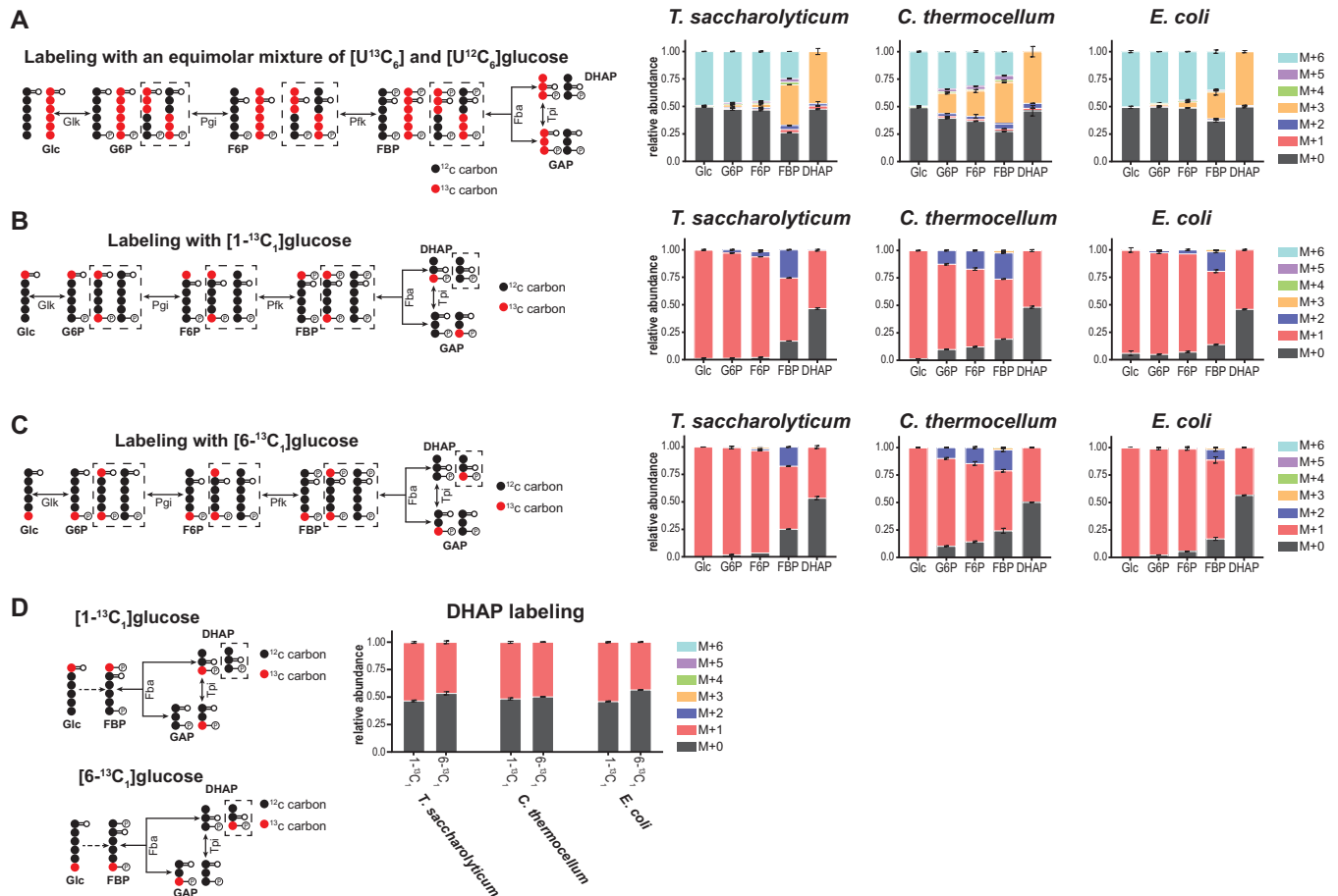
FIG 7 13 C labeling reveals reversibility of upper glycolytic reactions. (A, B, and C) Steady-state labeling patterns of upper glycolytic intermediates in C. thermocellum , T. saccharolyticum , and E. coli during anaerobic growth on an equimolar mixture of [U- 13 C 6 ]- and [U- 12 C 6 ]glucose (A), [1- 13 C 1 ]glucose (B), or [6- 13 C 1 ]glucose (C). The production of M + 3 FBP in panel A or M + 2 and M + 0 FBP in panels B and C indicated high reversibility of the Fba reaction in all three bacteria. Large differences in the reverse propagation of M + 3 FBP (A) or M + 2 and M + 0 FBP (B and C) to F6P suggested that the Pfk reaction was substantially more reversible in C. thermocellum than T. saccharolyticum or E. coli . (D) The reversibility of triose phosphate isomerase (Tpi) was revealed by [6- 13 C 1 ]glucose and [1- 13 C 1 ]glucose labeling. During [6- 13 C 1 ]glucose labeling, forward Fba activity first produces M + 0 DHAP. However, reverse Tpi flux results in the production of M + 1 DHAP from M + 1 GAP. Thus, the closer the M + 1 DHAP fraction is to 50%, the more reversible the Tpi. Labeling data indicated that Tpi was most reversible in C. thermocellum , with a proportion of M + 1 DHAP approaching 50% under both the [1- 13 C 1 ]glucose and [6- 13 C 1 ]glucose conditions. T. saccharolyticum had a less reversible Tpi reaction, followed by E. coli , which had a significant enrichment of M + 1 DHAP under the [1- 13 C 1 ]glucose condition and an enrichment of M + 0 DHAP under the [6- 13 C 1 ]glucose condition. The diagrams on the left depict predicted metabolite labeling. Solid arrows represent a single reaction; dashed arrows represent multiple reaction steps. 13 C-labeled carbons are colored red; 12 C-labeled carbons are colored black. Dashed boxes indicate metabolite-labeled forms produced by reverse flux. Data are averages from 2 or 3 independent biological replicates. Error bars show \pm SD.
