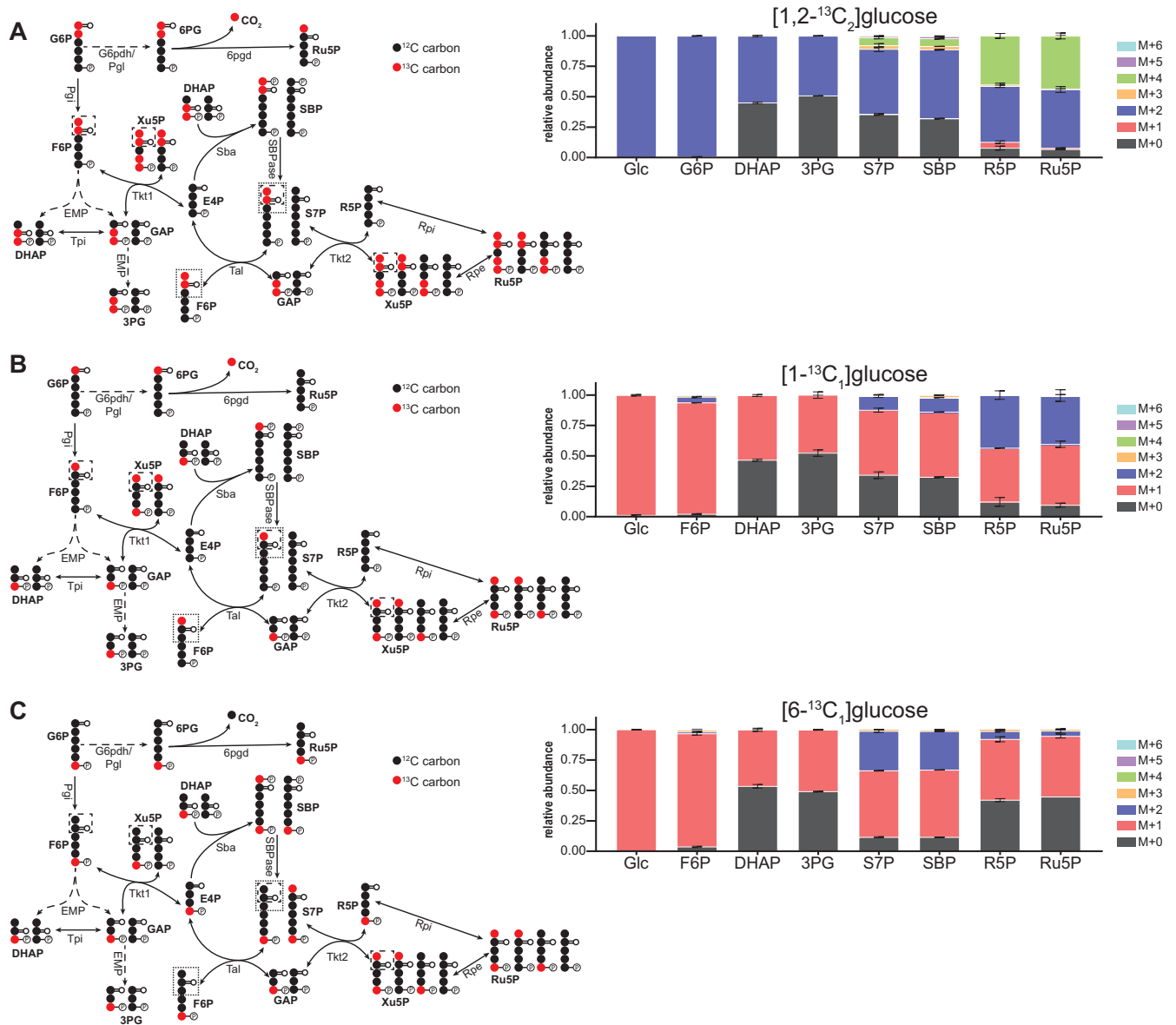
FIG 3 T. saccharolyticum has two nonoxidative routes for pentose phosphate production. Labeling of glycolytic and PPP intermediates when T. saccharolyticum was fed [1,2-^{13}\text{C}_2]\text{glucose} (A), [1-^{13}\text{C}_1]\text{glucose} (B), or [6-^{13}\text{C}_1]\text{glucose} (C). As described in the text, labeling patterns indicated that the oxidative branch of the PPP was essentially inactive and suggested the presence of a sedoheptulose biphosphate bypass, comprising SBP aldolase (Sba) and SBP phosphatase (SBPase). The diagrams on the left show predicted metabolite labeling with the specified isotope tracer. Solid arrows represent a single reaction; dashed arrows represent multiple reaction steps. Dotted boxes indicate carbons transferred during transaldolase and transketolase reactions. ^{13}\text{C} -labeled carbons are colored red; ^{12}\text{C} -labeled carbons are colored black. Data are averages from 2 or 3 independent biological replicates. Error bars show \pm SD. Abbreviations: 6PG, 6-phosphogluconate; 6pgd, 6-phosphogluconate dehydrogenase; E4P, erythrose-4-phosphate; G6pdh, glucose-6-phosphate dehydrogenase; R5P, ribose-5-phosphate; Rpe, ribose phosphate epimerase; Rpi, ribose phosphate isomerase; Ru5P, ribulose-5-phosphate; S7P, sedoheptulose-7-phosphate; Sba, sedoheptulose-1,7-bisphosphate aldolase; SBP, sedoheptulose-1,7-bisphosphate; SBPase, sedoheptulose-1,7-bisphosphate phosphatase; Tal, transaldolase; Tkt1, transketolase reaction 1; Tkt2, transketolase reaction 2; Xu5P, xylulose-5-phosphate.
