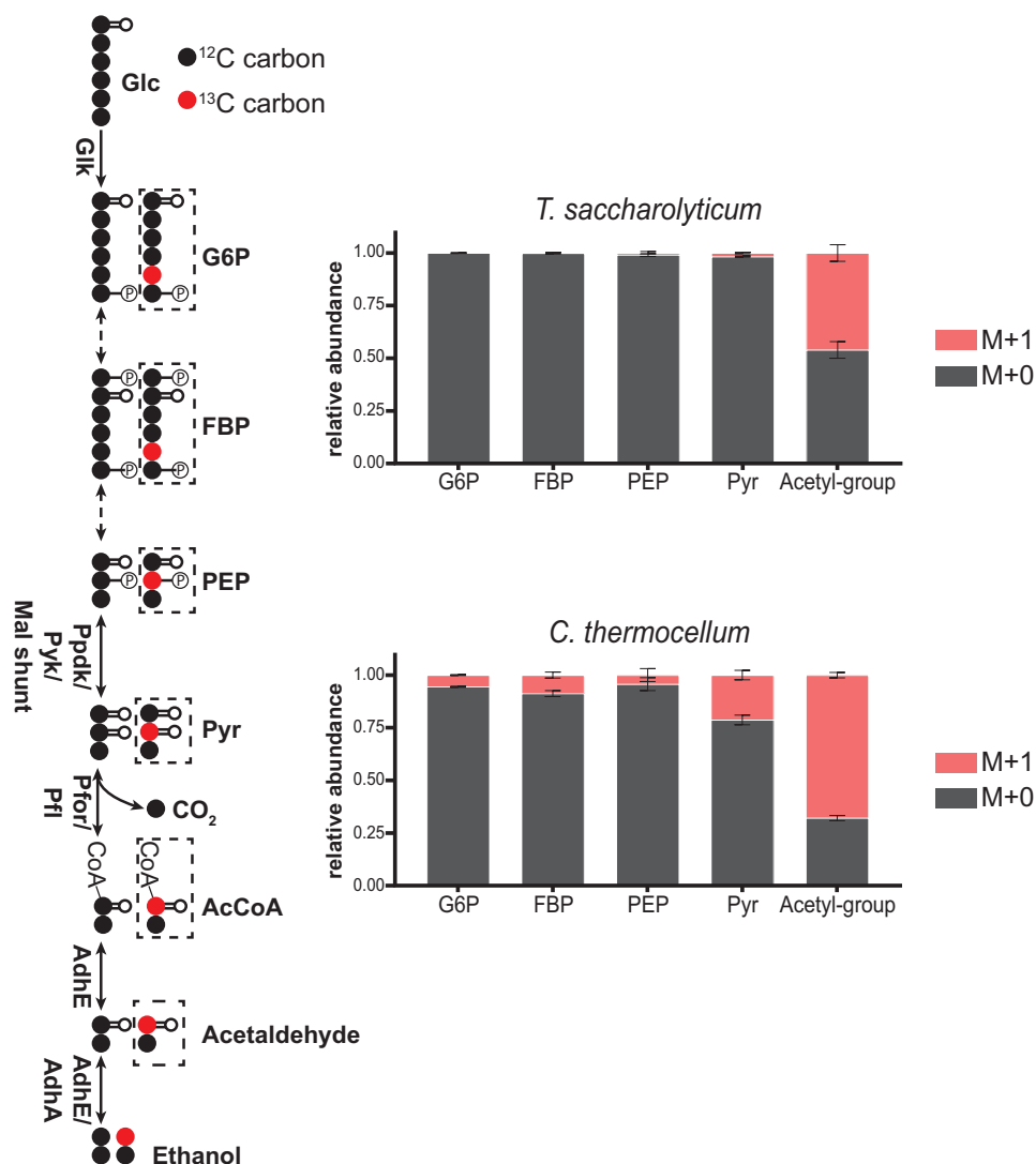
FIG 9 Reversibility of the pyruvate-to-ethanol pathway in C. thermocellum and T. saccharolyticum . Steady-state labeling with [1-^{13}\text{C}] ethanol in C. thermocellum and T. saccharolyticum revealed that the pyruvate-to-ethanol pathway in C. thermocellum was substantially more reversible than that of T. saccharolyticum . Reversibility of the AdhA and AdhE reactions resulted in ^{13}\text{C} -labeled AcCoA (at the acetyl group), which was more labeled in C. thermocellum than in T. saccharolyticum . Reverse activity of Pfor or Pfl resulted in the production of M + 1 pyruvate. Reverse activity of EMP reactions above pyruvate resulted in the production of labeled glycolytic intermediates. The diagrams on the left depict predicted metabolite labeling. Solid arrows represent a single reaction; dashed arrows represent multiple reaction steps. ^{13}\text{C} -labeled carbons are colored red; ^{12}\text{C} -labeled carbons are colored black. Dashed boxes indicate metabolite-labeled forms produced by reverse flux. Data are averages from 3 independent biological replicates. Error bars show \pm SD. Abbreviations: AdhA, alcohol dehydrogenase; AdhE, bifunctional alcohol/aldehyde dehydrogenase.
