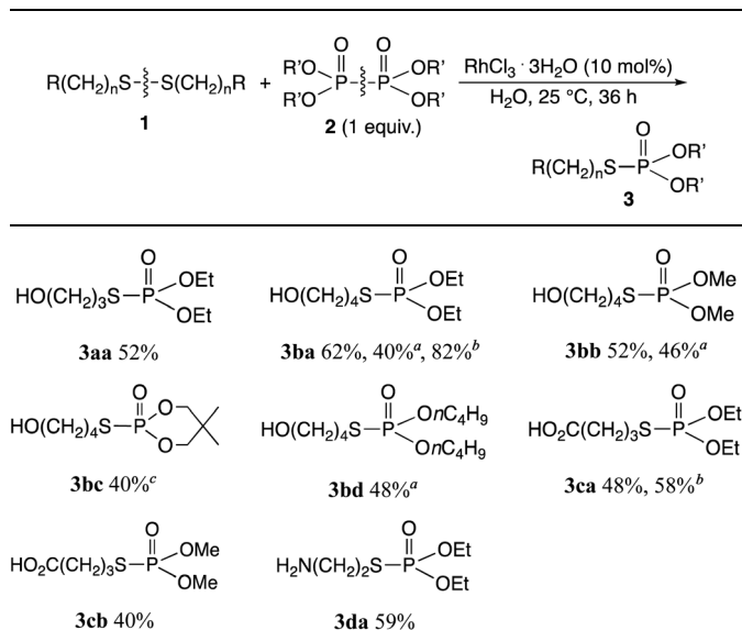
a At 40 °C for 36 h. b Use of \text{RhCl}_3 \cdot 3\text{H}_2\text{O} (20 mol%). c At 70 °C for 36 h.
