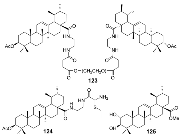
Fig. 37 Structure of UA derivatives 123 to 125.
