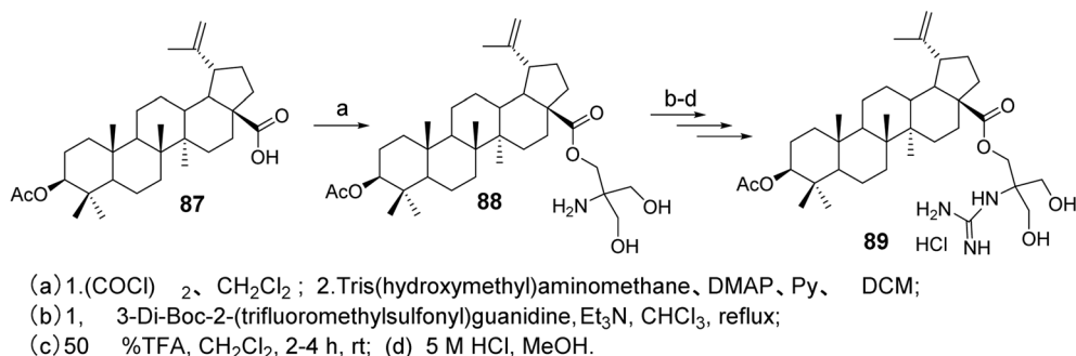
Fig. 26 Synthesis of BA derivative 89.
