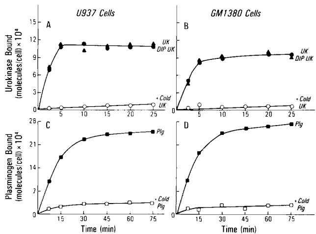
Figure 1. Time courses of ^{125} I-urokinase and ^{125} I-plasminogen binding to U937 and GM 1380 cells at 37°C. ^{125} I-UK in active or inactive (DIP-UK) form were added at 0.5 nM. Excess nonlabeled UK was used at 500 nM to assess the saturability of binding. ^{125} I-Plasminogen was added at 0.1 \mu M and nonlabeled plasminogen at 20 \mu M. For U937 cells, bound ligand from free ligand was separated by centrifugation through 20% sucrose. For the GM 1380 cells, the cell monolayer was washed by aspiration, and the bound ligand was extracted with SDS.
