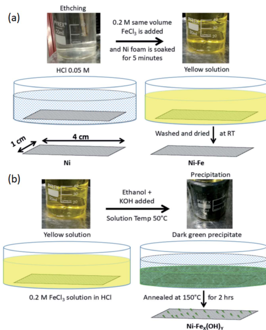
Fig. 1 (a) Preparation procedure for Ni-Fe samples. (b) Preparation procedure for Ni-Fe(OH) y samples.
