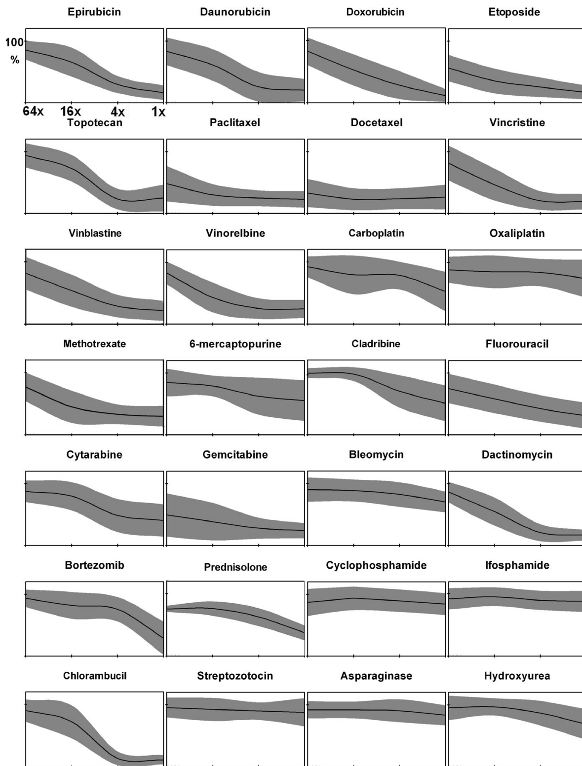
Figure 2 Mean values and standard deviations of drug sensitivity of 17 lymphoblastoid cell lines for 28 different cyto-static drugs. y axis: fraction of surviving cells 0–100% x axis: drug dilutions (1× represents the highest concentration).
