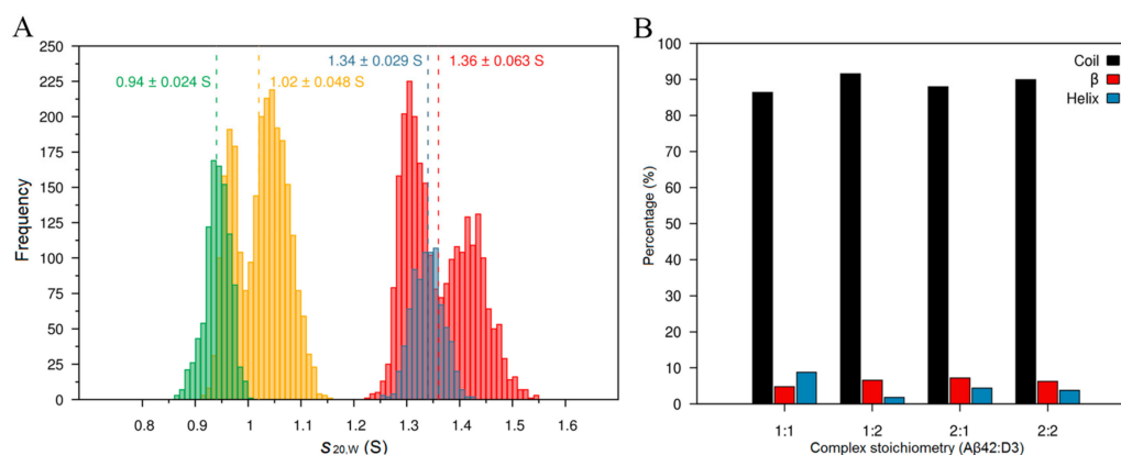
Figure 3. Sedimentation coefficient ( s_{20,w} ) distribution of D3 and A \beta 42 monomer complexes (A) and calculation of the secondary structure of A \beta 42 monomers in these complexes (B) based on MD simulations. The average s_{20,w} with standard deviations for the 1:1 (green), 2:1 (yellow), 1:2 (blue) and 2:2 (red) D3:A \beta 42 complexes are given for each complex above the corresponding histograms. Random coil, turns and bends are denoted as coil structures, while \beta -sheets and \beta -bridges are known as \beta -structures, and finally, \alpha -, 3_{10} - and \pi -helices, as helix structures.
