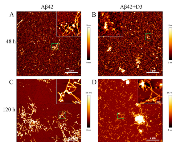
Figure 6. Atomic force microscopy (AFM) imaging to study the morphologies of 40 \mu\text{M} A \beta 42 in the absence (A and C) and presence (B and D) of 4 \mu\text{M} D3 in 20 mM sodium phosphate, 50 mM NaCl (pH 7.4—slightly alkali) at 20 °C after 48 h and 120 h of incubation. The imaging was carried out at room temperature in air, using AC mode. Inserts show amplifications of areas marked with green squares. The scale bars are 2 \mu\text{m} for the overviews and 200 nm for the inserts.
