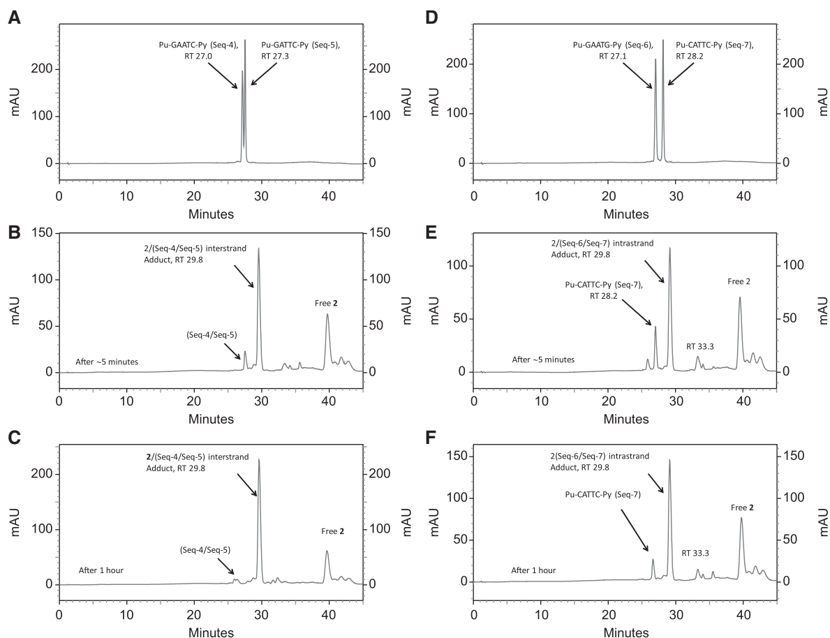
Figure 4. HPLC chromatograms; (A) Annealed Pu-GAATC-Py duplex ( Seq-4/Seq-5 ); (B) Immediately (i.e. ~5 min) after mixing DRG-16 ( 2 ) with the Seq-4/Seq-5 duplex showing appearance of the 2/( Seq-4/Seq-5 ) interstrand adduct at RT 29.8 min; (C) 1 h after mixing 2 with the Seq-4/Seq-5 duplex followed by incubation at room temperature showing completion of reaction; (D) Annealed Pu-GAATG-Py duplex ( Seq-6/Seq-7 ); (E) Immediately (~5 min) after mixing DRG-16 ( 2 ) with the Seq-6/Seq-7 duplex showing appearance of the intrastrand 2/( Seq-6/Seq-7 ) duplex adduct at RT 29.8 min and a small amount of monoalkylated adduct at RT 33.3 min; (F) 1 h after mixing 2 with the Seq-6/Seq-7 duplex showing the reaction nearing completion.
