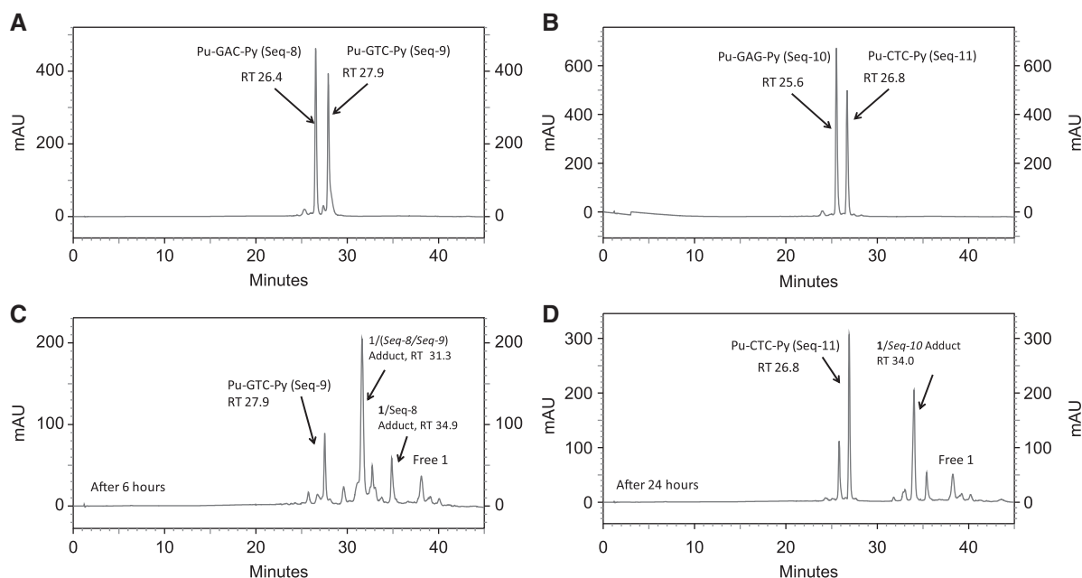
Figure 3. HPLC chromatograms; (A) Annealed Pu-GAC-Py duplex ( Seq-8/Seq-9 ); (B) Annealed Pu-GAG-Py duplex ( Seq-10/Seq-11 ); (C) 6 hours after incubation of SJG-136 ( 1 ) with the Seq-8/Seq-9 duplex showing appearance of the 1/(Seq-8/Seq-9) interstrand cross-linked adduct at RT 31.3 min and a small amount of 1/(Seq-8) monoalkylated adduct at RT 34.9 min (resulting from partial denaturation of 1/(Seq-8/Seq-9) ), (D) 24 h after incubation of SJG-136 ( 1 ) with the Seq-10/Seq-11 duplex showing appearance of the 1/Seq-10 monoalkylated adduct at RT 34.0 min resulting from complete denaturation of the initially formed 1/(Seq-10/Seq-11) .
