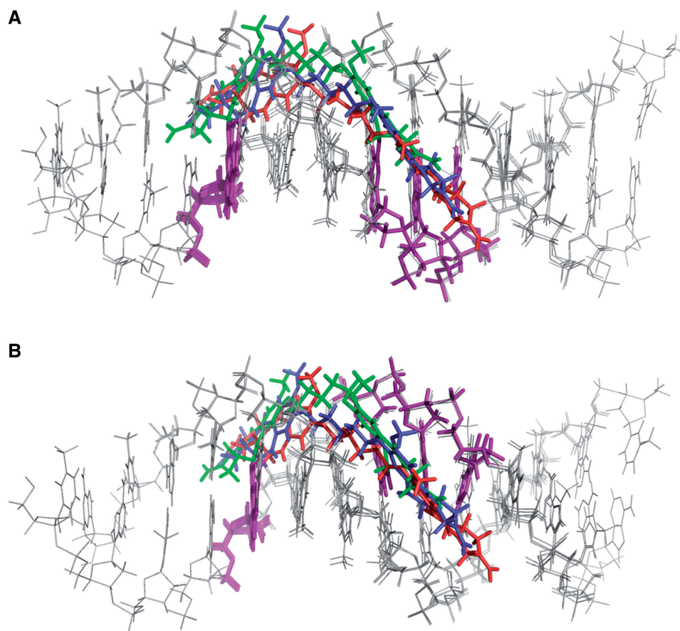
Figure 8. Overlay of energy minimised molecular models of the different types of covalent cross-linked adducts formed by DRG-16 ( 2 ) with the duplex oligonucleotides of different lengths and cross-linking potential (i.e. inter- versus intrastrand): ( A ) DRG-16 interstrand cross-linking with Pu-GATC-Py (green ligand), Pu-GAATC-Py (blue ligand) and Pu-GAAATC-Py (red ligand) duplex oligonucleotides; ( B ) DRG-16 intrastrand cross-linking with Pu-GATG-Py (green ligand), Pu-GAATG-Py (blue ligand) and Pu-GAAATG-Py (red ligand) duplex oligonucleotides. Note: In both figures the covalently bound guanine bases are highlighted in purple.
