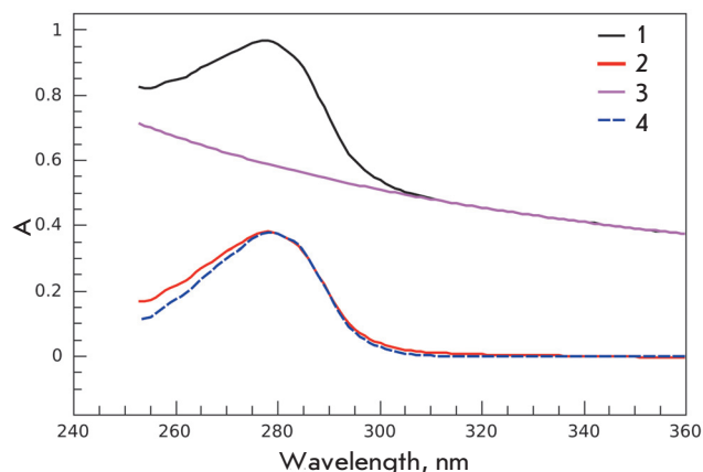
Fig. 3. Absorption spectra of a S1(A1) preparation (1 mg/ml), stored at 4 °C at low ionic strength (20 mM Hepes, pH 7.3, 1 mM \text{MgCl}_2 ) measured before (1) and after (2) addition of KCl up to a concentration of 100 mM. Curve 3 was obtained by extrapolation of the long-wavelength part of S1(A1) absorption spectrum into its short-wavelength region, and it reflects light-scattering of the S1(A1) preparation at low ionic strength in the entire wavelength range. Curve 4 was obtained by subtracting curve 3 from curve 1.
