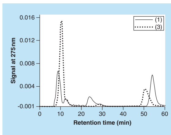
Figure 5. Size-exclusion chromatography profiles of aliquots of reaction mixtures containing chondroitin sulfate type A, \text{Cu}^{2+} and (1) (solid line) or (3) (dotted line). The reaction mixtures contained 1 mM (1) or (3), 8 mg/ml chondroitin sulfate type A and 0.1 mM \text{Cu}^{2+} and were kept at 37°C overnight.
