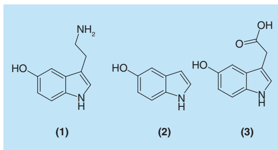
Figure 1. Chemical structures of the compounds used in this study. (1) serotonin, (2) 5-hydroxyindole and (3) 5-hydroxyindole-3-acetic acid.
