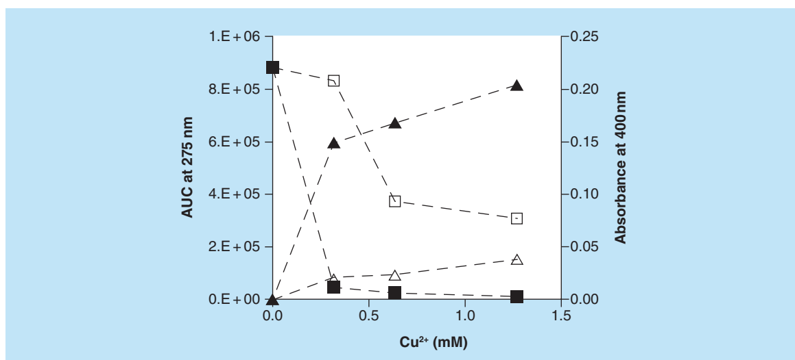
Figure 3. Effect of \text{Cu}^{2+} concentration on reactions containing (1), chondroitin sulfate type A and \text{Cu}^{2+} . AUC corresponding to (1) for reactions with (closed squares) or without (open squares) CS A and absorbance at 400 nm of the reaction mixtures with (closed triangles) or without (open triangles) CS A. The reaction mixtures contained 1 mM (1), 2.5 mg/ml CS A and between 0 and 1.3 mM \text{Cu}^{2+} and were incubated overnight at 37°C. CS A: Chondroitin sulfate type A.
