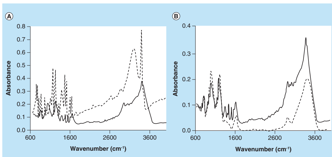
Figure 14. Fourier transform IR scans of the pigment made from (2) and fucoidan (solid line in both panels) and (2) (dashed line in panel A) or fucoidan (dashed line in panel B).
