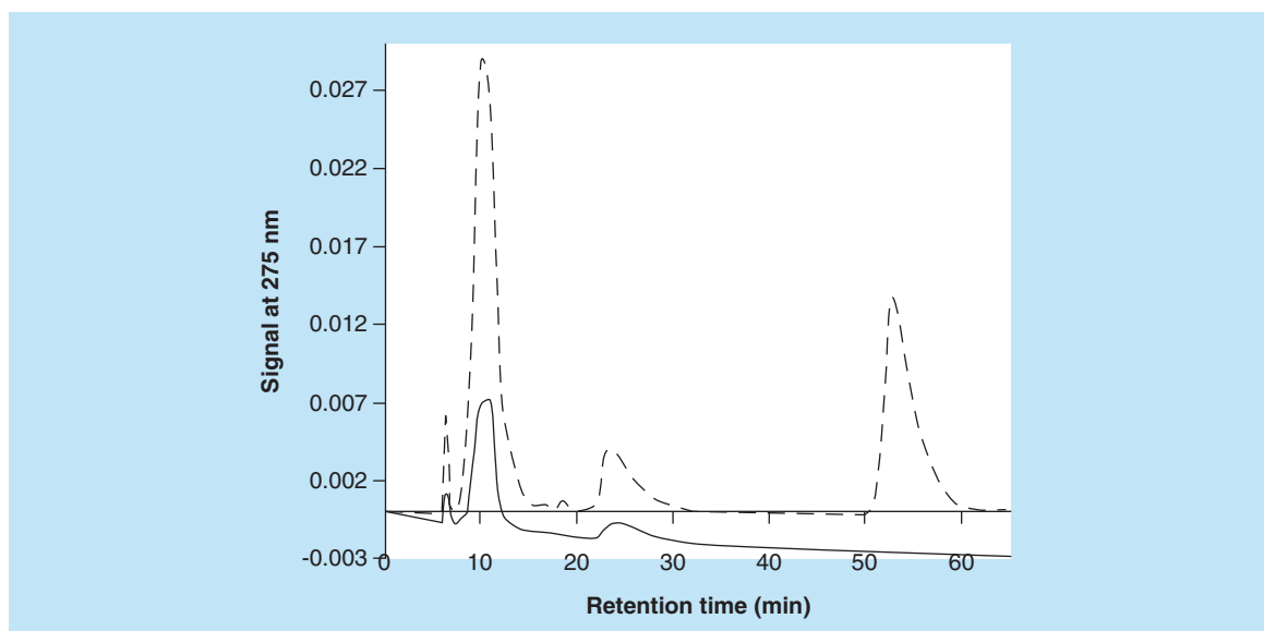
Figure 9. Size-exclusion chromatography profiles of diluted aliquots from the reaction mixture (dotted line) shown in Figure 8, panel A and the reaction mixture after dialysis against water (solid line).
