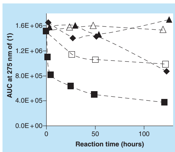
Figure 6. Kinetic profile of the AUC (signal at 275 nm) corresponding to (1) as determined by size-exclusion chromatography analysis. Reaction mixtures contained 2 mM (1) and 0 (open symbols) or 0.05 (closed symbols) mM \text{Cu}^{2+} and 0 mg/ml polysaccharides (triangles), 4 mg/ml chondroitin sulfate type A (diamonds) or 4 mg/ml fucoidan (squares).
