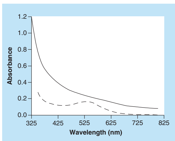
Figure 12. UV-Vis spectra of reaction mixtures involving (2) and fucoidan (solid line) and (3) and chondroitin sulfate type C (dashed line) from the reaction mixtures shown in Figures 10 & 11, respectively.
