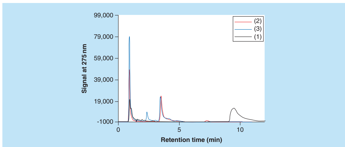
Figure 2. Reverse phase-HPLC profiles of aliquots of reaction mixtures containing chondroitin sulfate type A, \text{Cu}^{2+} and (1) (black line), (2) (red line) or (3) (blue line). The reaction mixtures contained 1 mM (1), (2) or (3), 8 mg/ml chondroitin sulfate type A and 0.1 mM \text{Cu}^{2+} and were kept at 37°C overnight.
