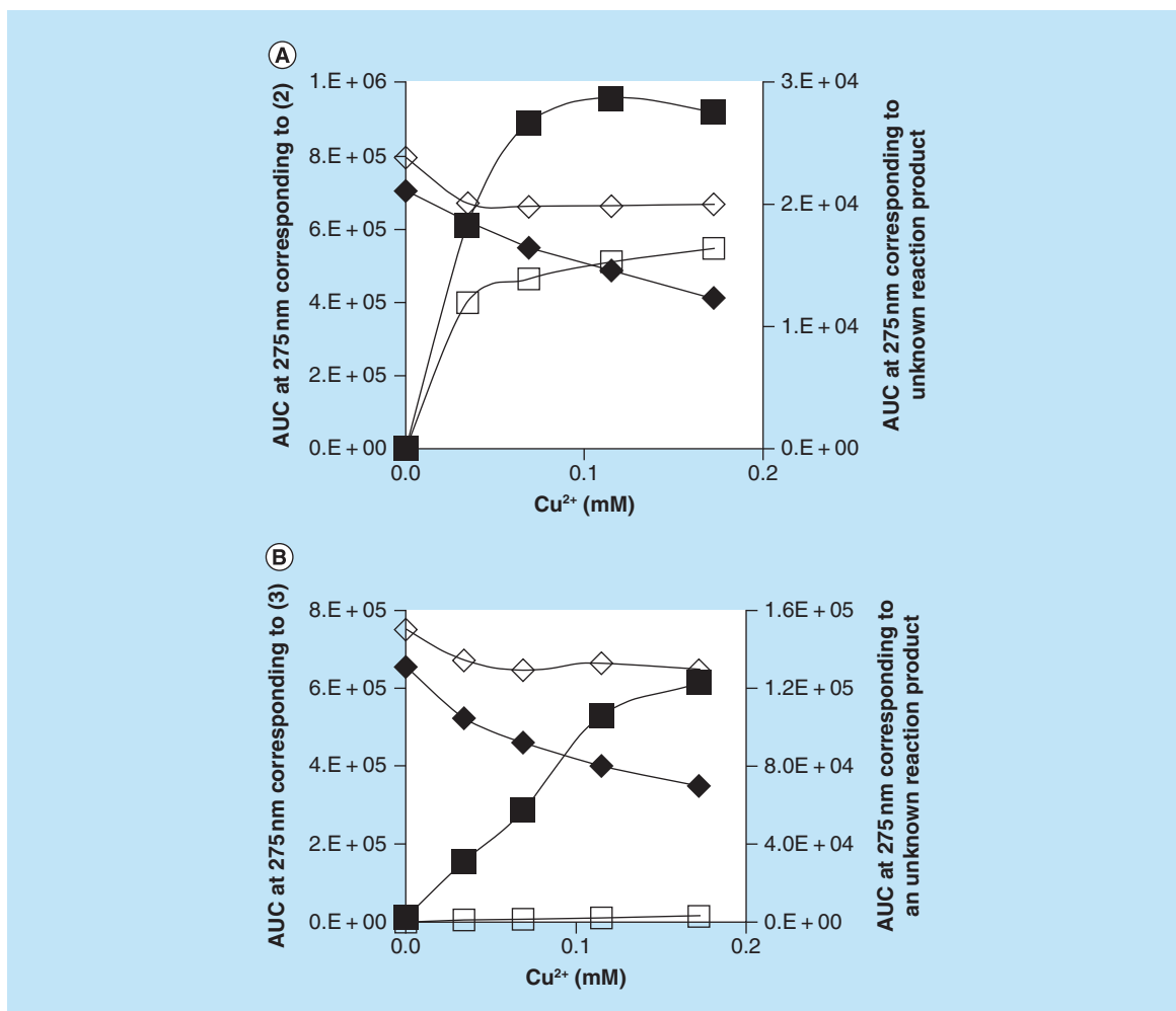
Figure 4. Effect of \text{Cu}^{2+} on reactivity of (2) and (3). Effect of \text{Cu}^{2+} concentration on the reaction between (2) (panel A) or (3) (panel B), CS A and \text{Cu}^{2+} . AUC corresponding to (2) or (3) (diamonds) for reactions with (closed symbols) or without (open symbols) CS A and AUC corresponding to an unknown reaction product (squares) as a function of \text{Cu}^{2+} concentration present. The reaction mixtures contained 1 mM (2) or (3), 0 or 8 mg/ml CS A and between 0 and 0.17 mM \text{Cu}^{2+} and were incubated overnight at 37°C. CS A: Chondroitin sulfate type A.
