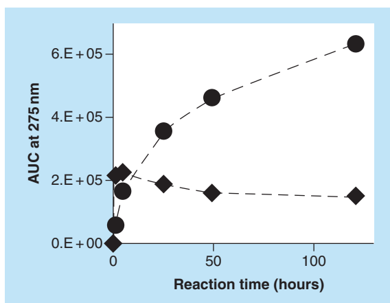
Figure 7. Kinetic profile of the AUC (signal at 275 nm), as determined by size-exclusion chromatography analysis, corresponding to fucoïdan (circles) and unknown reaction product (diamonds). The reaction mixture contained 2 mM (1), 0.05 mM \text{Cu}^{2+} and 4 mg/ml fucoïdan.
