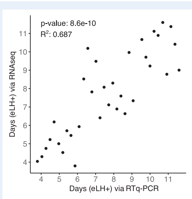
Figure 6. Correlation of predicted time points from RTq-PCR data versus predictions from RNA-seq data of six panel genes. eLH+, estimated LH+.
