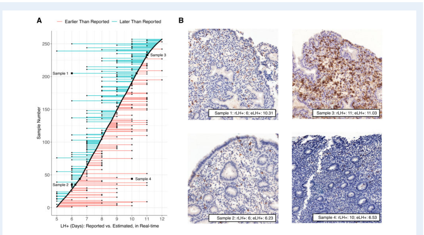
Figure 7. Identification of mistimed samples. (A) Samples shown in order identified by EndoTime (y-axis). EndoTime times shown as smooth curve. Deviations of reported timings from EndoTime timings shown as coloured horizontal lines. (B) Bright-field imaging with staining by the uNK marker CD56 for four samples. These images can be used to verify the progress of tissue development as earlier time points are associated with simple and tubular glands, while corkscrew-shaped glands are associated with biopsies donated during later time points. Samples 2 and 4 appear to be early samples, while Sample 1 and 3 are late samples. EndoTime estimates are consistent with this. Reported timings agree for Sample 2 and 3 but are discrepant for Sample 1 and 4 by about four days. eLH+, estimated LH+.
