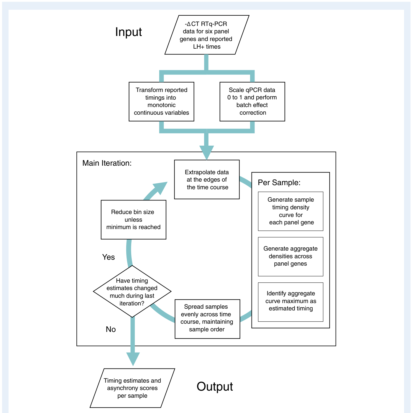
Figure 2. Estimation of endometrial sample timings by EndoTime. Pre-processing steps normalize and apply minor batch correction to -\Delta\text{CT} qPCR gene expression data and transform reported sample timings, in LH+, into a continuous domain suitable for modelling. The bulk of the computation is an iterative process of binning data, generating an aggregate pseudo-density curve per sample, the maxima of which are selected as an estimate for the most likely sample timings, and assessment of the relative difference in sample estimates between one iteration and the preceding one. Once the difference in estimates falls below a predefined threshold value, diminishing returns are considered to have been reached and the modelling process ceases, returning the final sample timing estimates and an associated values for asynchrony, which reflect the degree to which all six panel genes agree upon estimates.
