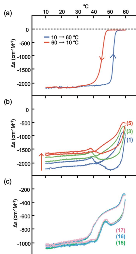
Fig. 4 \Delta\epsilon (375 nm)/temperature profiles from experiments of heating and cooling of ( M )-1/( P )-2 (1 : 1) at a constant rate of 1 \text{ }^{\circ}\text{C min}^{-1} between 10 and 60 ^{\circ}\text{C} , shown by (a) in 30% water-THF (10 \mu\text{M} ); (b) in 33% water-THF (10 \mu\text{M} ) starting from -2000 \text{ cm}^{-1} \text{ M}^{-1} ; (c) enlarged view of (b). The number of heating/cooling cycles is shown in parentheses in (b) and (c). See Fig. S17† for details.
