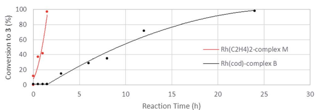
Fig. 7 Kinetic profiles of complexes B and M as catalysts in parallel dialkynylation reactions of 1 with diphenylacetylene.
