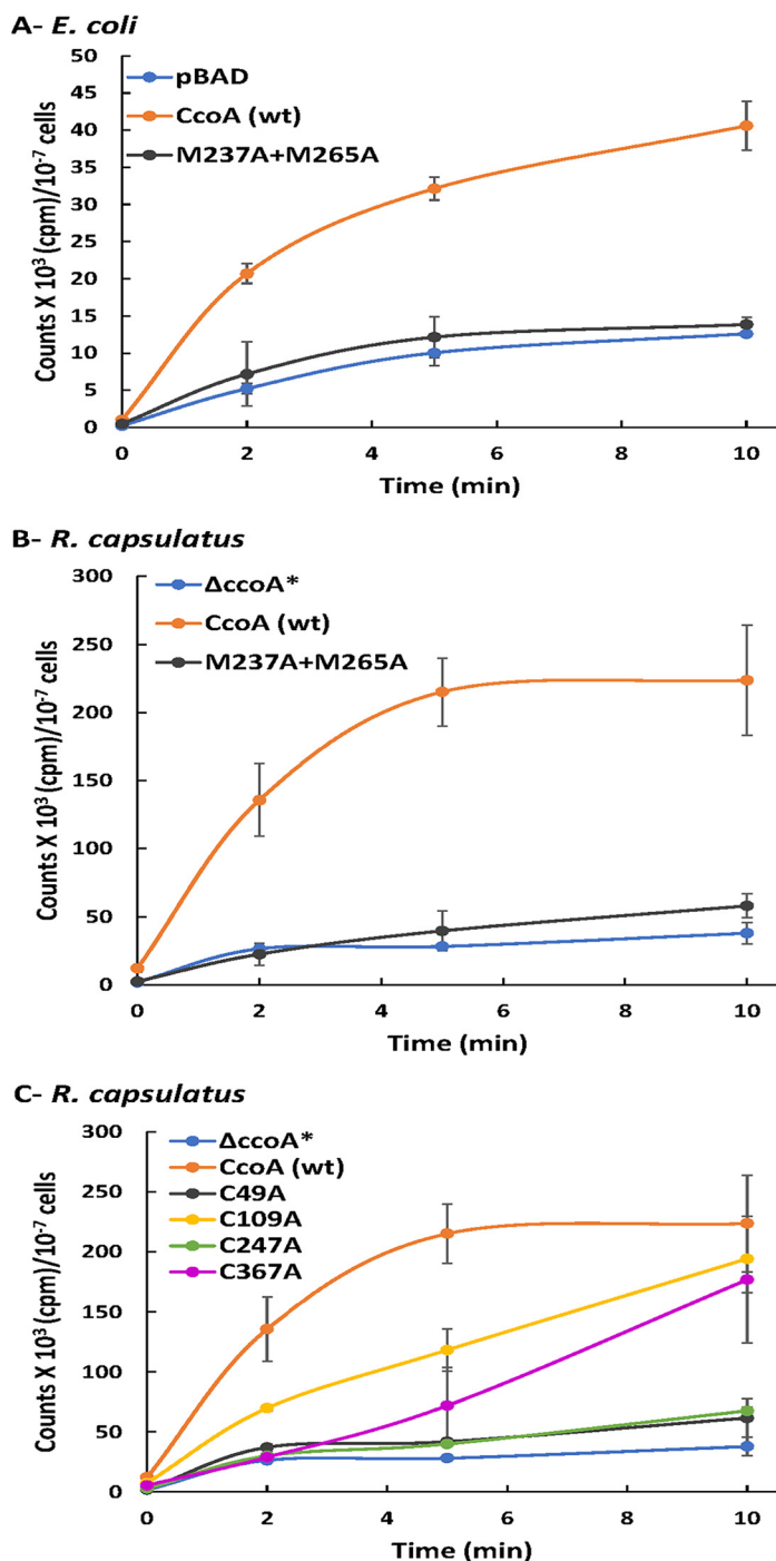
FIG 3 Whole-cell radioactive ^{64}\text{Cu} uptake by CcoA M_{237}A+M_{265}A double and Cys single mutant derivatives. (A to C) ^{64}\text{Cu} uptake kinetics observed with the CcoA M_{237}A+M_{265}A double mutant and C_{49}A , C_{109}A , C_{247}A , and C_{367}A single mutants using appropriate L-ara induced E. coli (LMG194) (A) and R. capsulatus \Delta ccoA^* ( \Delta ccoA \Delta copA , SE24) (B and C) cells, expressing L-ara-inducible native and mutant ccoA alleles. pBAD and \Delta ccoA refer to control strains, as appropriate. Uptake assays were performed as described in Materials and Methods. Activities measured in cells kept on ice were subtracted from those measured in cells incubated at 37°C, and assays were repeated at least three times using multiple independent cultures. CcoA (wt) refers to ( \Delta ccoA +plasmid-borne ccoA ) strain carrying L-ara-inducible native CcoA, where \Delta ccoA^* is \Delta ccoA \Delta copA (SE24), used to avoid frequent CopA revertants seen with a ccoA deletion (see Table S1) (12). Error bars correspond to the standard deviations around the mean values. In each case, at least three biological and three technical repeats were performed.
