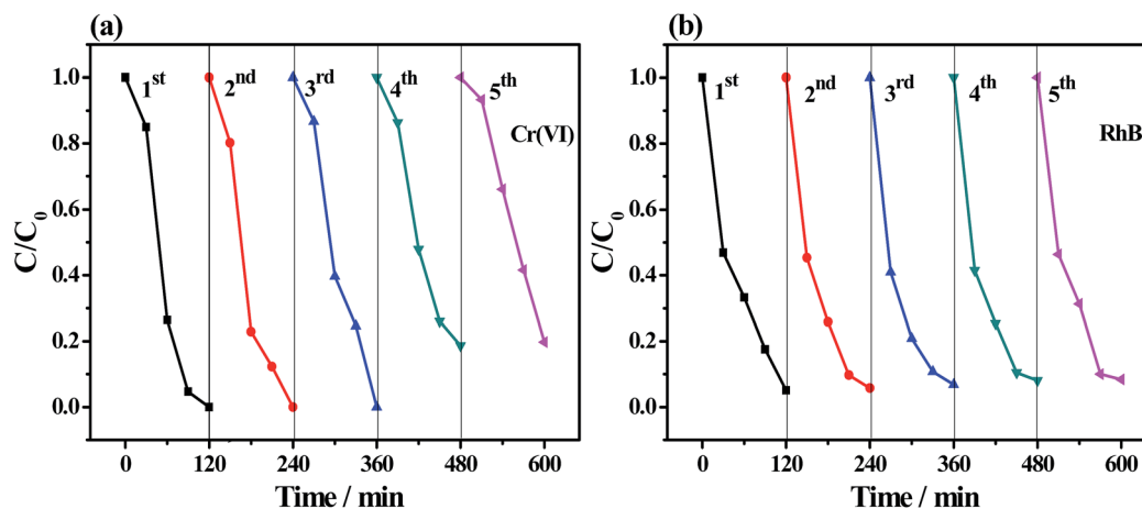
Fig. 9 Recycled test of \text{Bi}_2\text{S}_3 @NM-100 for (a) photocatalytic reduction of Cr(vi) (initial concentration: 10 \text{ mg L}^{-1} , photocatalyst dosage: 200 \text{ mg L}^{-1} , \text{pH} = 3.0 ) and (b) photocatalytic degradation of RhB (initial concentration: 20 \text{ mg L}^{-1} , photocatalyst dosage: 200 \text{ mg L}^{-1} , \text{pH} = 7.0 ).
