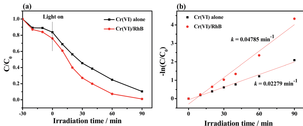
Fig. 8 Photocatalytic reduction (a) and reduction kinetics of Cr(vi) (b) with and without RhB using \text{Bi}_2\text{S}_3 @NM-100 sample (initial concentrations of Cr(vi): 10 \text{ mg L}^{-1} and RhB: 5 \text{ mg L}^{-1} , photocatalyst dosage: 200 \text{ mg L}^{-1} , \text{pH} = 3.0 ).
