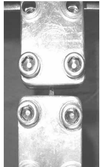
Figure 4 – Test body (tendon) mounted on the mechanical testing machine.
