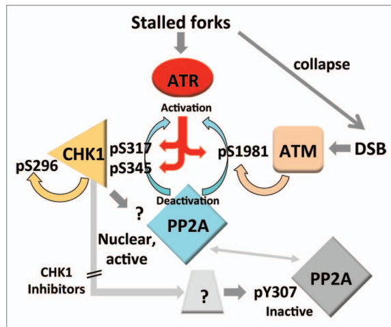
Figure 1. Pathways that can contribute to cancer cell survival. Replication stress activates the ATR pathway, leading to activation of CHK1 through phosphorylation of Ser345 and Ser317; Ser296 is autophosphorylated and serves as a marker of activated CHK1. ATR also phosphorylates ATM on Ser1981. CHK1 activity is required for active nuclear PP2A. Inhibition or depletion of CHK1 decreases nuclear PP2A and increases (through unknown mechanisms) an inhibitory phosphorylation of PP2A on Tyr307. Inhibition of PP2A results in enhanced phosphorylation of CHK1 on Ser235 and S296 and ATM on Ser1981. Basal signals that activate ATM may come from ATR acting at replication forks that are stalled at natural barriers or, after collapse of stalled forks, auto-activation by DNA double-strand breaks.
