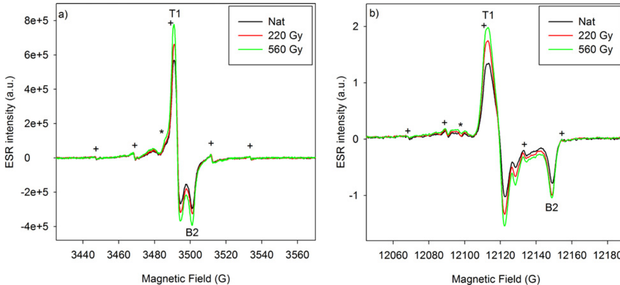
Fig 3. X-band (a) and Q-band (b) spectra of the powder sample #3 (natural aliquot + two irradiated aliquots). Acquisition parameters are provided in Table 1. Sweep width is of 145 G for all ESR spectra. Key: (*) identifies the \text{SO}_2^- component. The multiplet centered at g = 2.0033 (labelled as “+”) is an isotropic and non-radiosensitive signal due to a dimethyl radical [9,21], and the signal at g = 2.0115 is probably associated to a \text{CO}_3^- radical [36].
